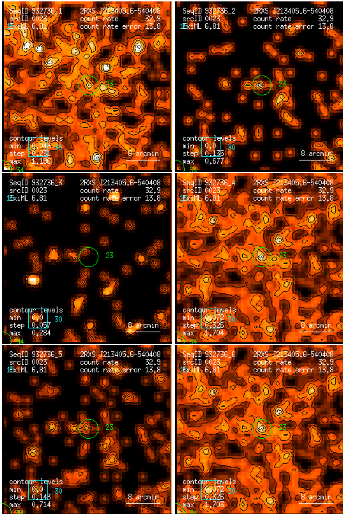
Figure 23: RASS 932736: detection 0023: band rate images, Gaussian filter: (1) PSPC channels 11 – 41, (2) 52 – 90, (3) 91 – 201, (4) 11 – 235, (5) 52 – 201, (6) 11 – 201. Broad band rates in counts/ks. Band rate contour levels in counts/ks/arcmin 2 .
