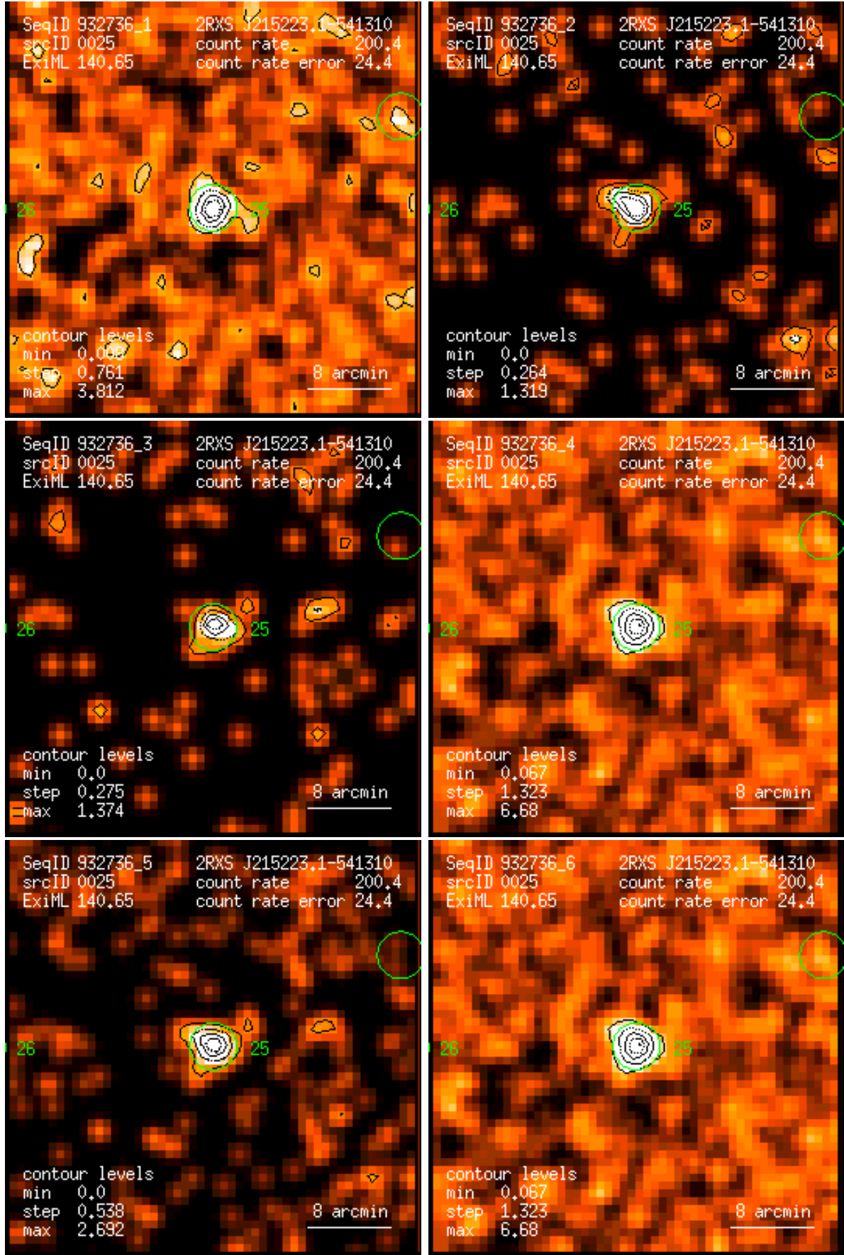
Figure 25: RASS 932736: detection 0025: band rate images, Gaussian filter: (1) PSPC channels 11 – 41, (2) 52 – 90, (3) 91 – 201, (4) 11 – 235, (5) 52 – 201, (6) 11 – 201. Broad band rates in counts/ks. Band rate contour levels in counts/ks/arcmin 2 .
