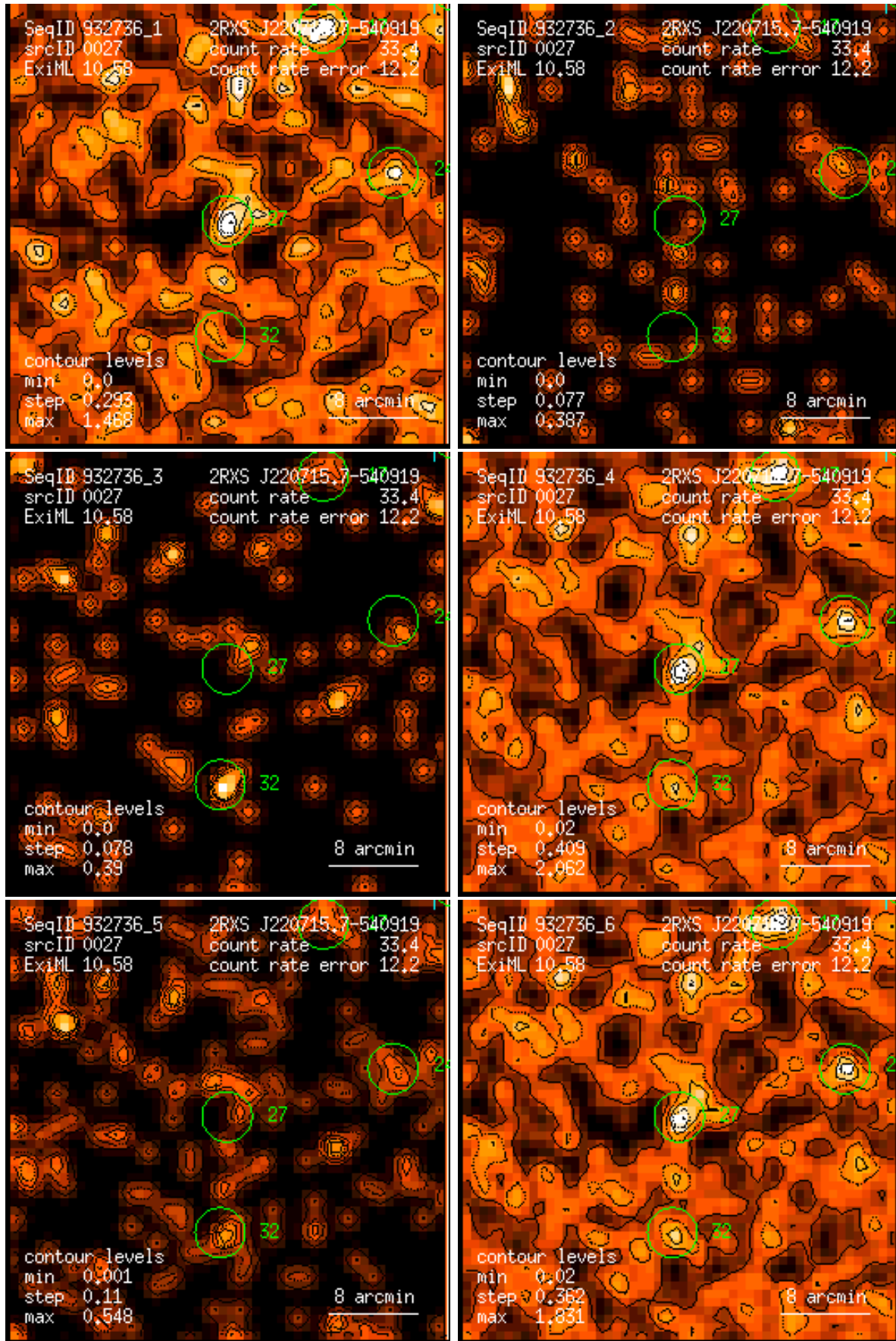
Figure 27: RASS 932736: detection 0027: band rate images, Gaussian filter: (1) PSPC channels 11 – 41, (2) 52 – 90, (3) 91 – 201, (4) 11 – 235, (5) 52 – 201, (6) 11 – 201. Broad band rates in counts/ks. Band rate contour levels in counts/ks/arcmin 2 .
