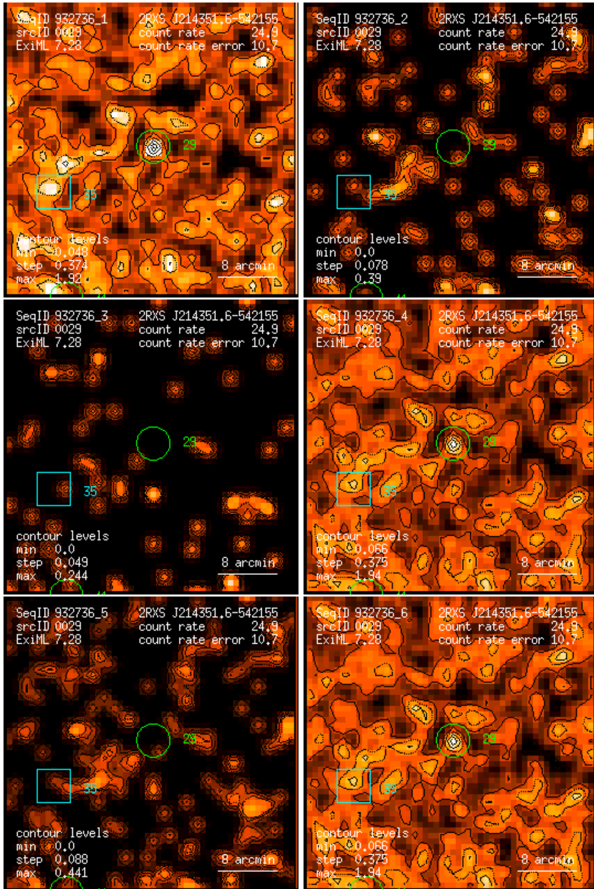
Figure 29: RASS 932736: detection 0029: band rate images, Gaussian filter: (1) PSPC channels 11 – 41, (2) 52 – 90, (3) 91 – 201, (4) 11 – 235, (5) 52 – 201, (6) 11 – 201. Broad band rates in counts/ks. Band rate contour levels in counts/ks/arcmin 2 .
