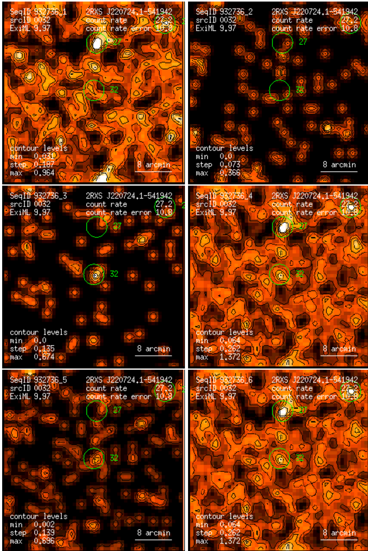
Figure 32: RASS 932736: detection 0032: band rate images, Gaussian filter: (1) PSPC channels 11 – 41, (2) 52 – 90, (3) 91 – 201, (4) 11 – 235, (5) 52 – 201, (6) 11 – 201. Broad band rates in counts/ks. Band rate contour levels in counts/ks/arcmin 2 .
