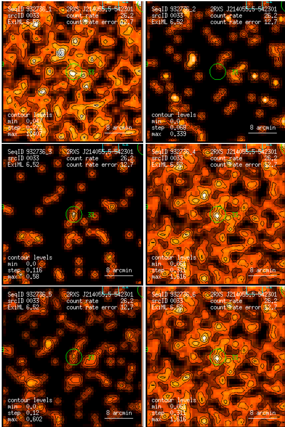
Figure 33: RASS 932736: detection 0033: band rate images, Gaussian filter: (1) PSPC channels 11 – 41, (2) 52 – 90, (3) 91 – 201, (4) 11 – 235, (5) 52 – 201, (6) 11 – 201. Broad band rates in counts/ks. Band rate contour levels in counts/ks/arcmin 2 .
