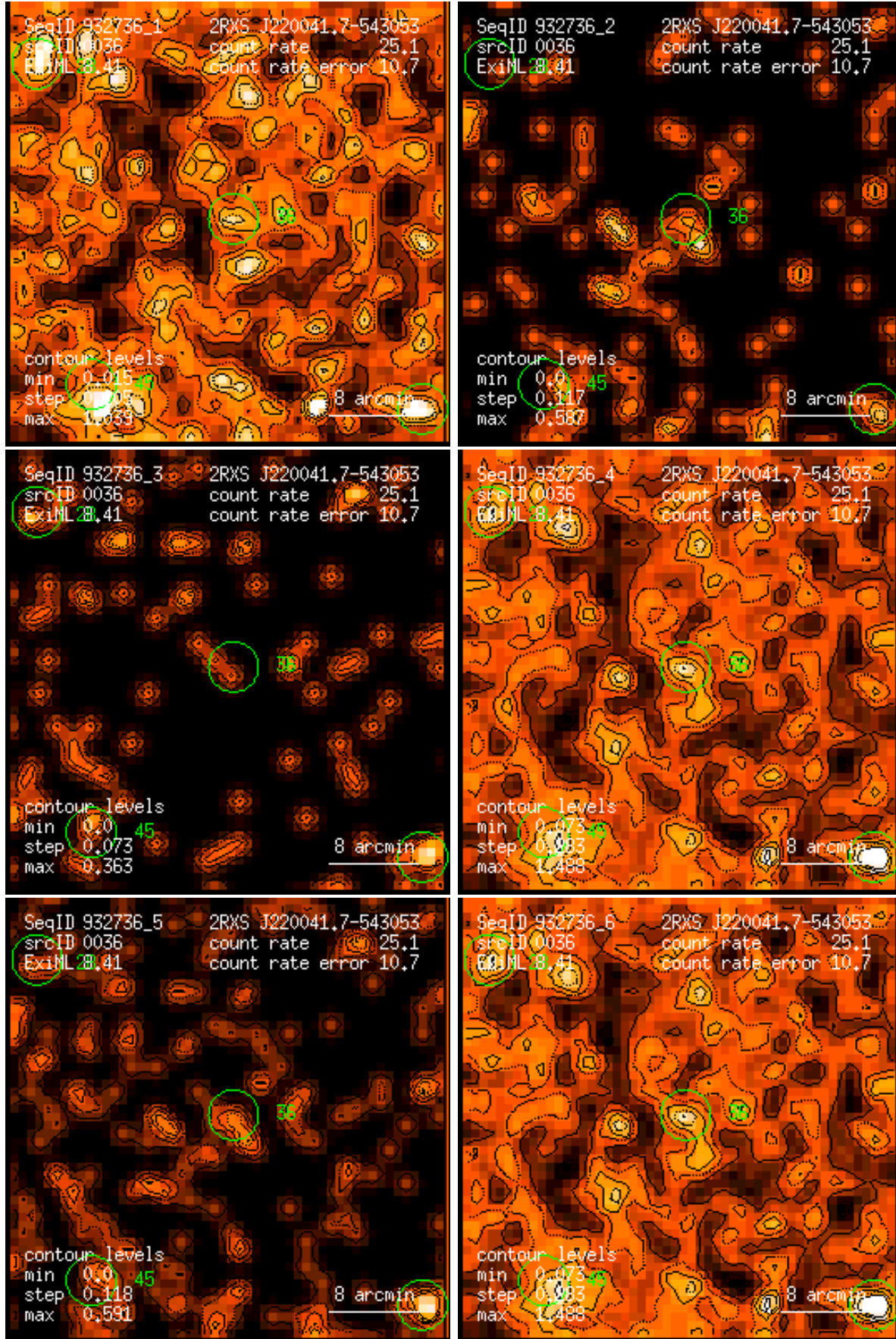
Figure 36: RASS 932736: detection 0036: band rate images, Gaussian filter: (1) PSPC channels 11 – 41, (2) 52 – 90, (3) 91 – 201, (4) 11 – 235, (5) 52 – 201, (6) 11 – 201. Broad band rates in counts/ks. Band rate contour levels in counts/ks/arcmin 2 .
