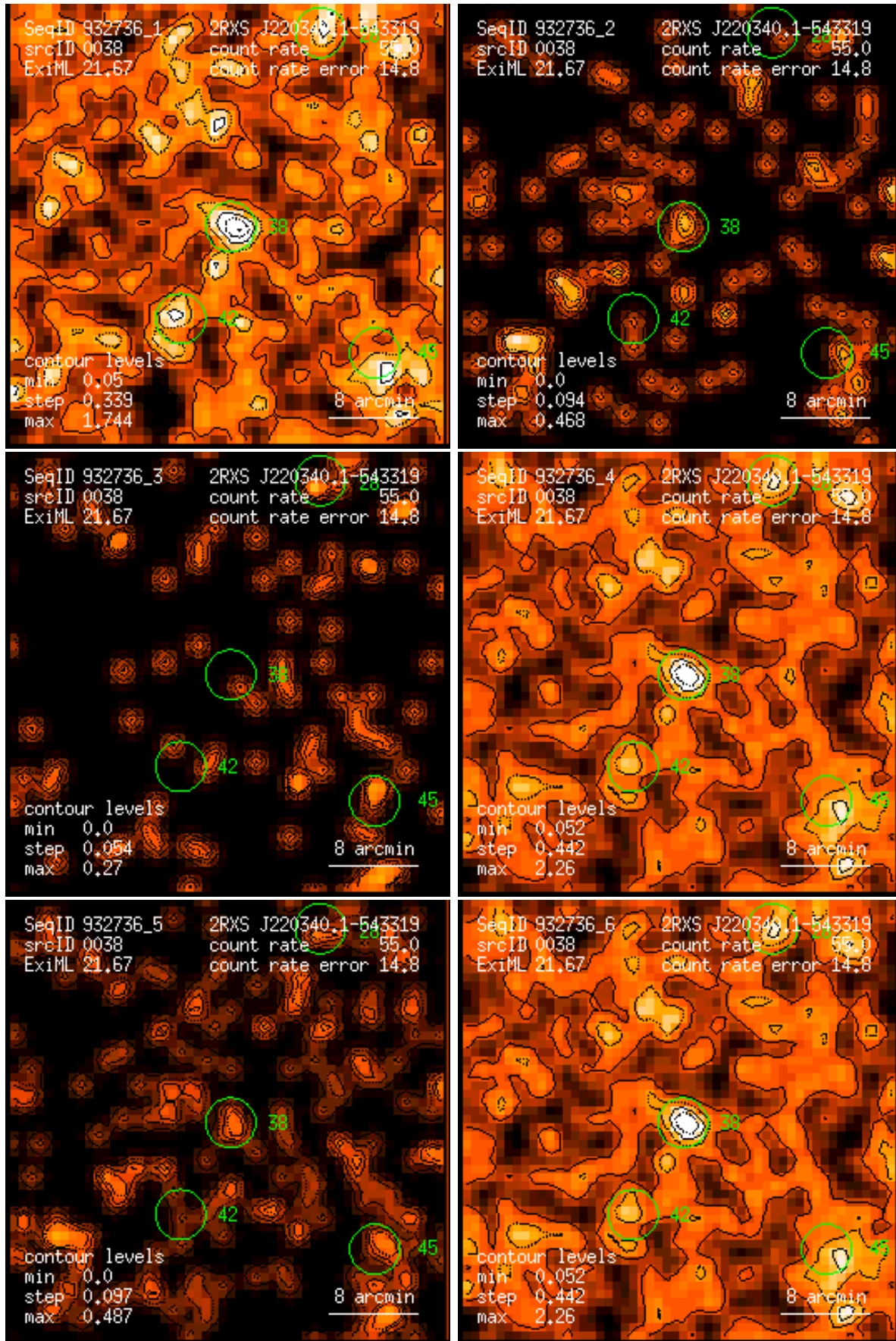
Figure 38: RASS 932736: detection 0038: band rate images, Gaussian filter: (1) PSPC channels 11 – 41, (2) 52 – 90, (3) 91 – 201, (4) 11 – 235, (5) 52 – 201, (6) 11 – 201. Broad band rates in counts/ks. Band rate contour levels in counts/ks/arcmin 2 .
