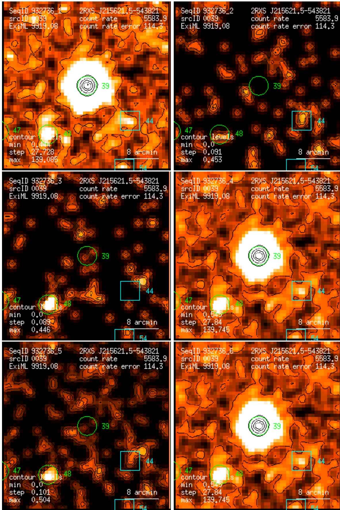
Figure 39: RASS 932736: detection 0039: band rate images, Gaussian filter: (1) PSPC channels 11 – 41, (2) 52 – 90, (3) 91 – 201, (4) 11 – 235, (5) 52 – 201, (6) 11 – 201. Broad band rates in counts/ks. Band rate contour levels in counts/ks/arcmin 2 .
