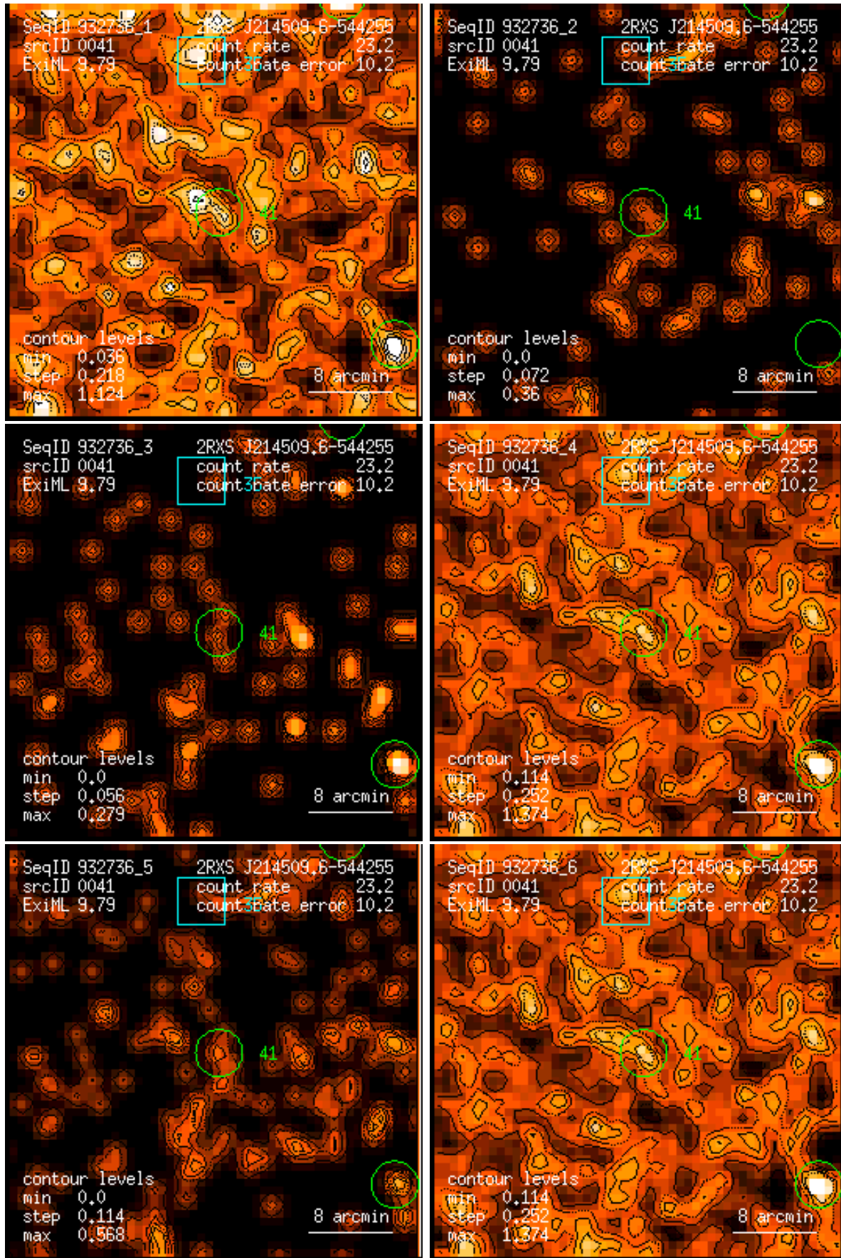
Figure 41: RASS 932736: detection 0041: band rate images, Gaussian filter: (1) PSPC channels 11 – 41, (2) 52 – 90, (3) 91 – 201, (4) 11 – 235, (5) 52 – 201, (6) 11 – 201. Broad band rates in counts/ks. Band rate contour levels in counts/ks/arcmin 2 .
