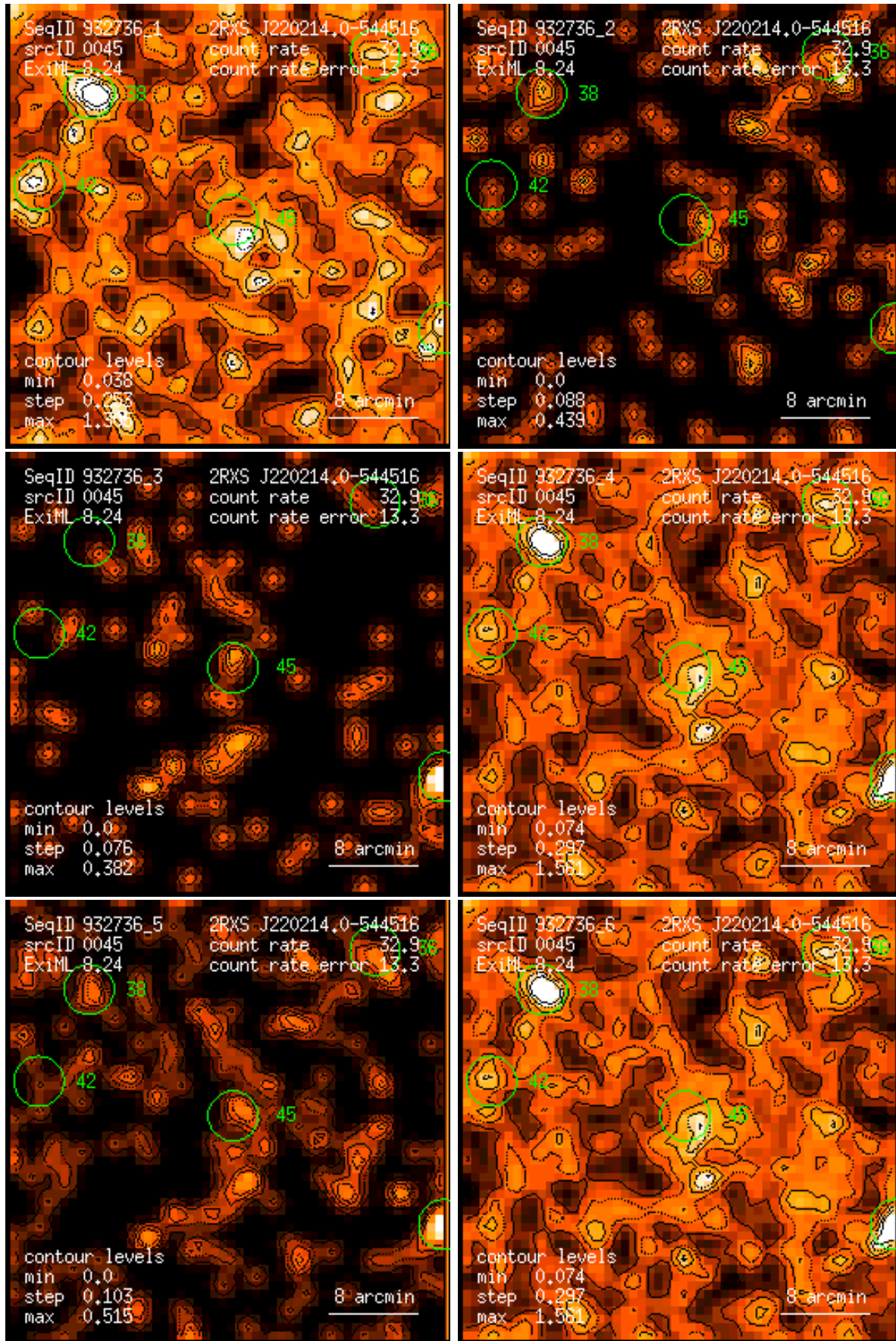
Figure 45: RASS 932736: detection 0045: band rate images, Gaussian filter: (1) PSPC channels 11 – 41, (2) 52 – 90, (3) 91 – 201, (4) 11 – 235, (5) 52 – 201, (6) 11 – 201. Broad band rates in counts/ks. Band rate contour levels in counts/ks/arcmin 2 .
