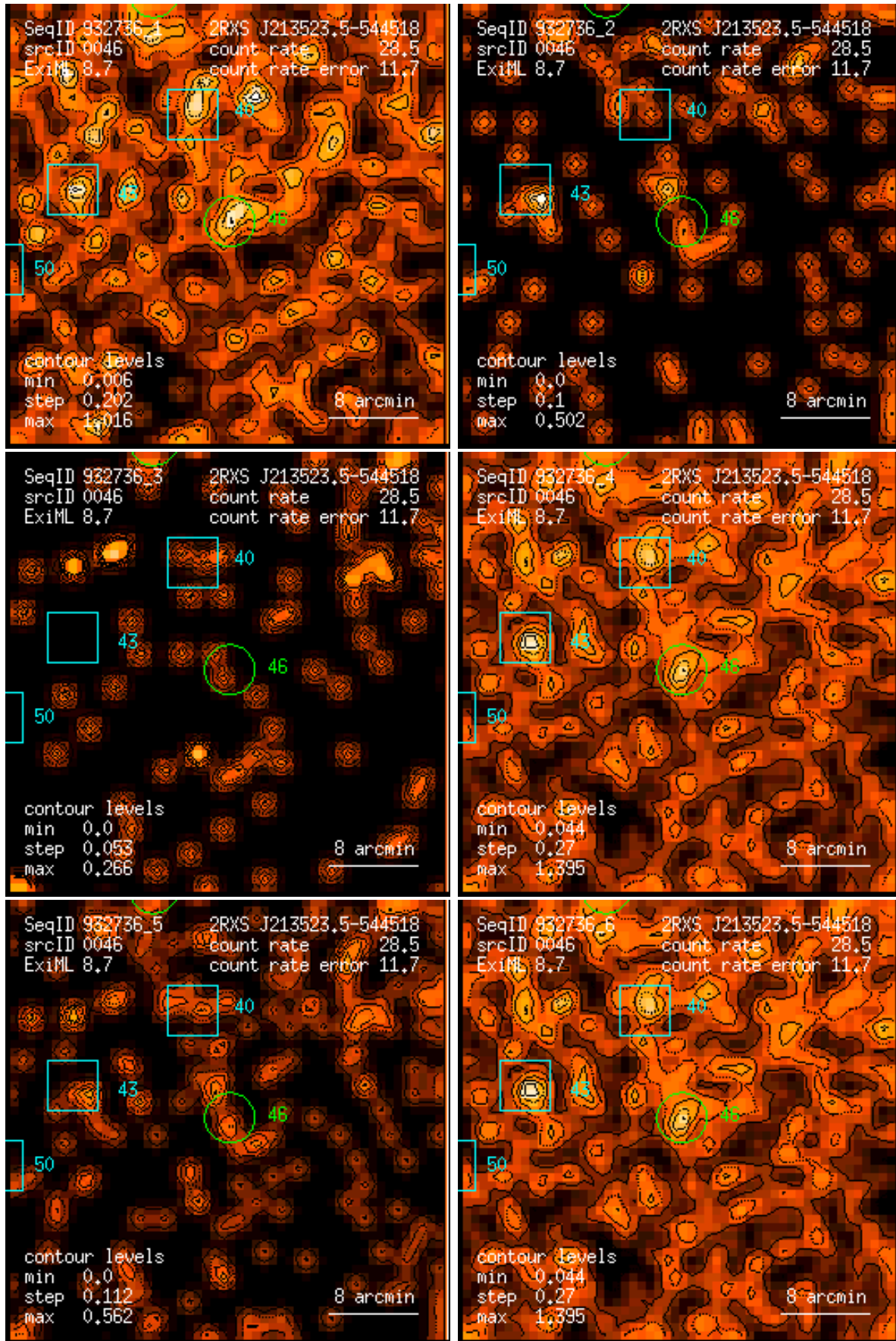
Figure 46: RASS 932736: detection 0046: band rate images, Gaussian filter: (1) PSPC channels 11 – 41, (2) 52 – 90, (3) 91 – 201, (4) 11 – 235, (5) 52 – 201, (6) 11 – 201. Broad band rates in counts/ks. Band rate contour levels in counts/ks/arcmin 2 .
