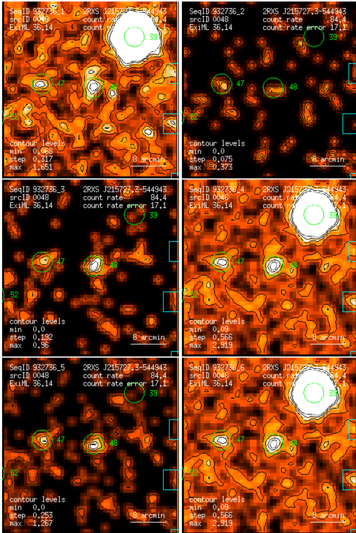
Figure 48: RASS 932736: detection 0048: band rate images, Gaussian filter: (1) PSPC channels 11 – 41, (2) 52 – 90, (3) 91 – 201, (4) 11 – 235, (5) 52 – 201, (6) 11 – 201. Broad band rates in counts/ks. Band rate contour levels in counts/ks/arcmin 2 .
