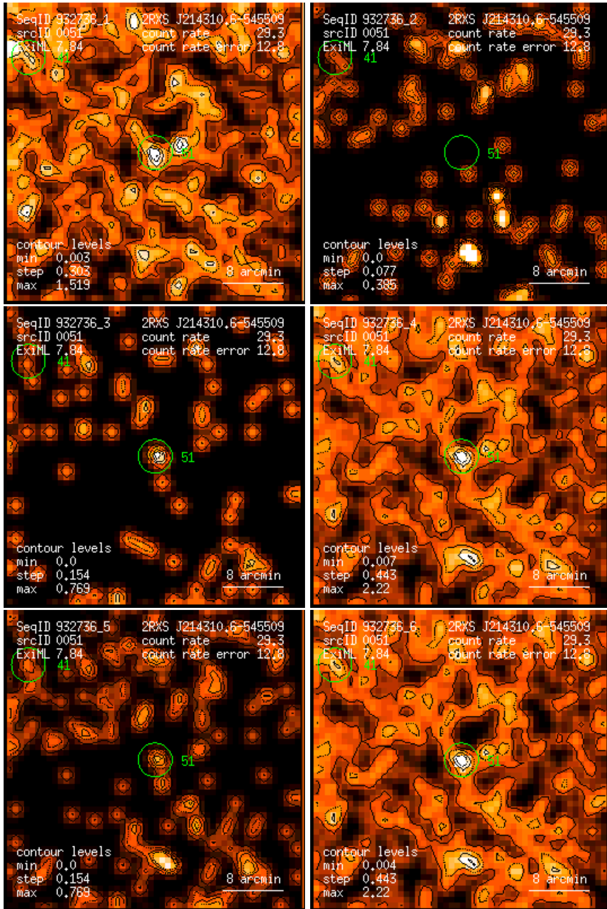
Figure 51: RASS 932736: detection 0051: band rate images, Gaussian filter: (1) PSPC channels 11 – 41, (2) 52 – 90, (3) 91 – 201, (4) 11 – 235, (5) 52 – 201, (6) 11 – 201. Broad band rates in counts/ks. Band rate contour levels in counts/ks/arcmin 2 .
