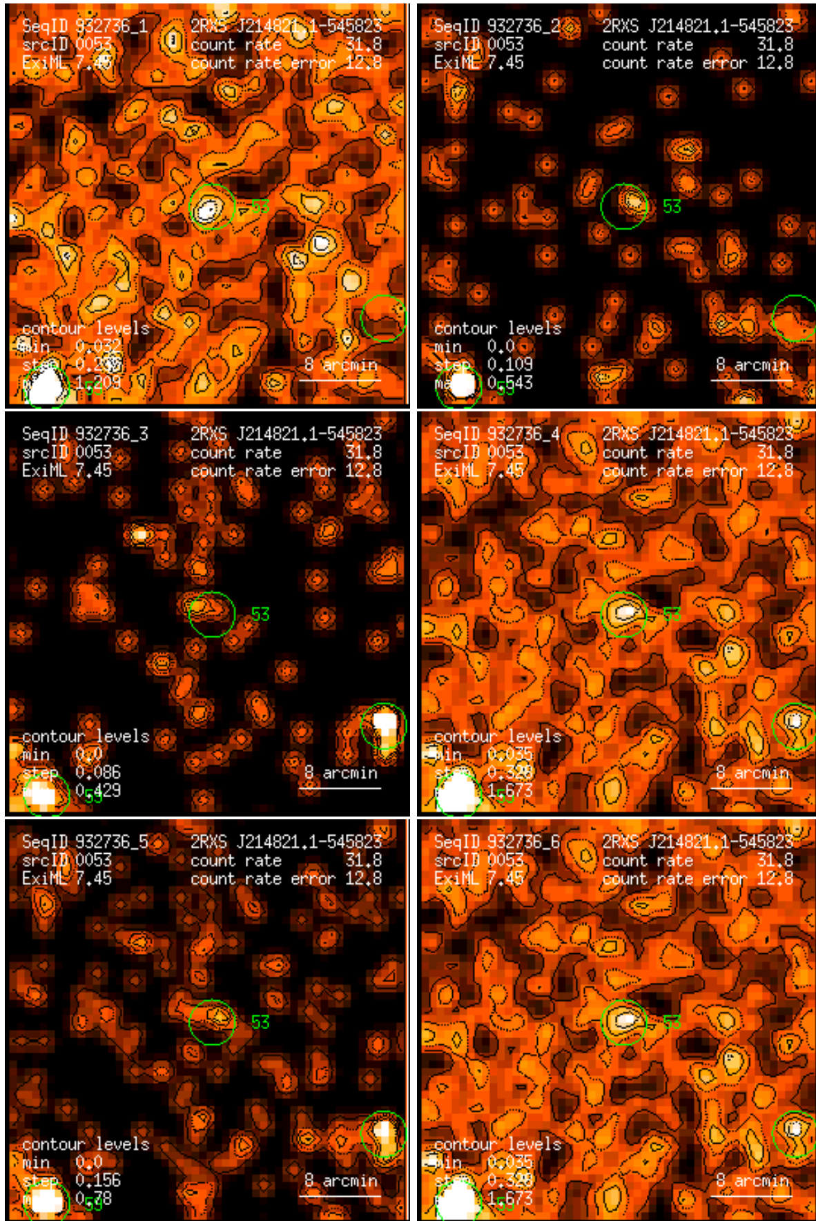
Figure 53: RASS 932736: detection 0053: band rate images, Gaussian filter: (1) PSPC channels 11 – 41, (2) 52 – 90, (3) 91 – 201, (4) 11 – 235, (5) 52 – 201, (6) 11 – 201. Broad band rates in counts/ks. Band rate contour levels in counts/ks/arcmin 2 .
