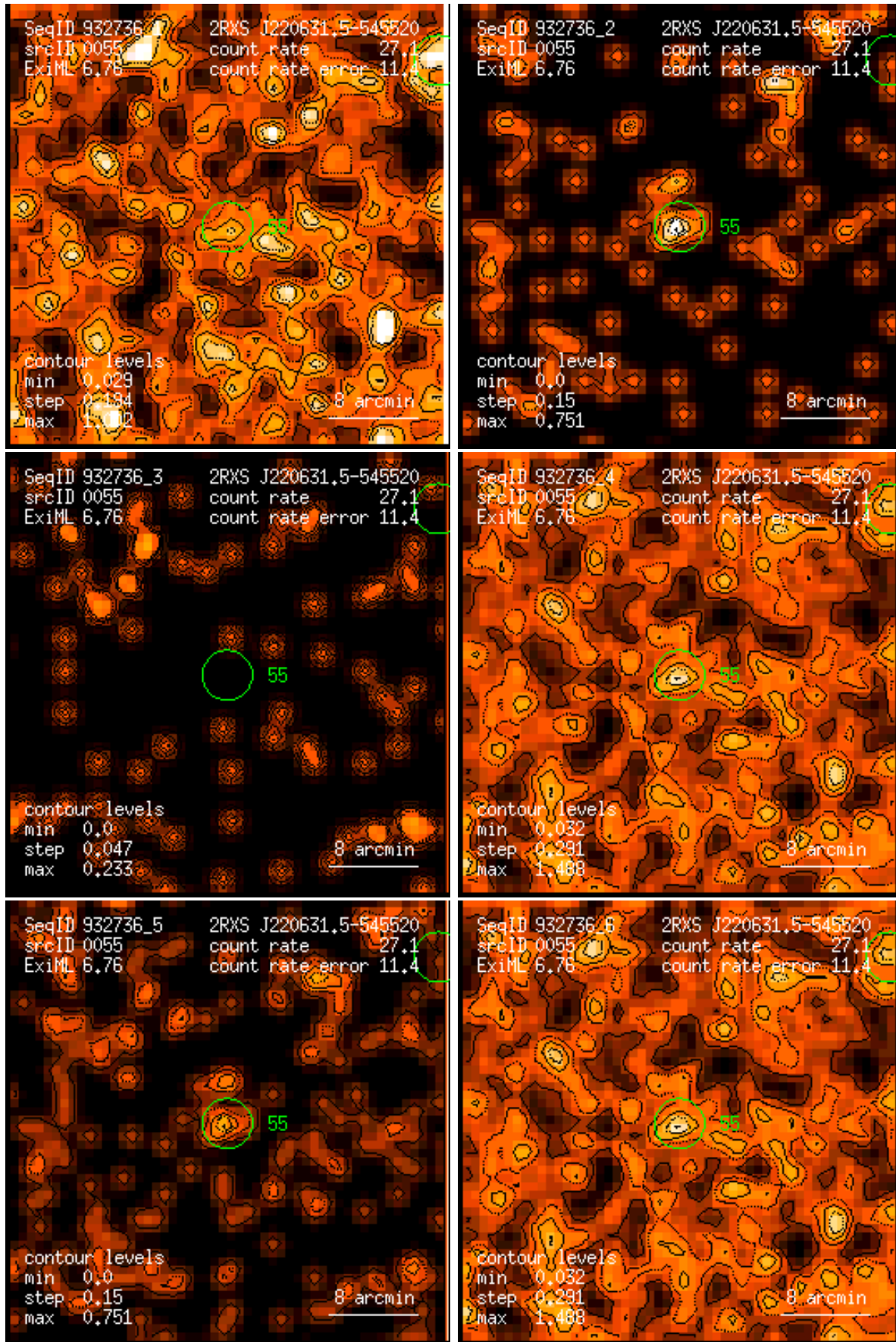
Figure 55: RASS 932736: detection 0055: band rate images, Gaussian filter: (1) PSPC channels 11 – 41, (2) 52 – 90, (3) 91 – 201, (4) 11 – 235, (5) 52 – 201, (6) 11 – 201. Broad band rates in counts/ks. Band rate contour levels in counts/ks/arcmin 2 .
