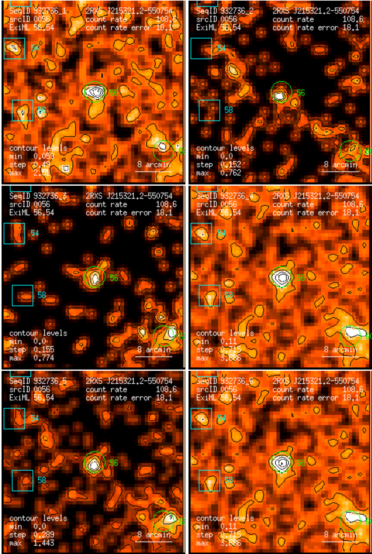
Figure 56: RASS 932736: detection 0056: band rate images, Gaussian filter: (1) PSPC channels 11 – 41, (2) 52 – 90, (3) 91 – 201, (4) 11 – 235, (5) 52 – 201, (6) 11 – 201. Broad band rates in counts/ks. Band rate contour levels in counts/ks/arcmin 2 .
