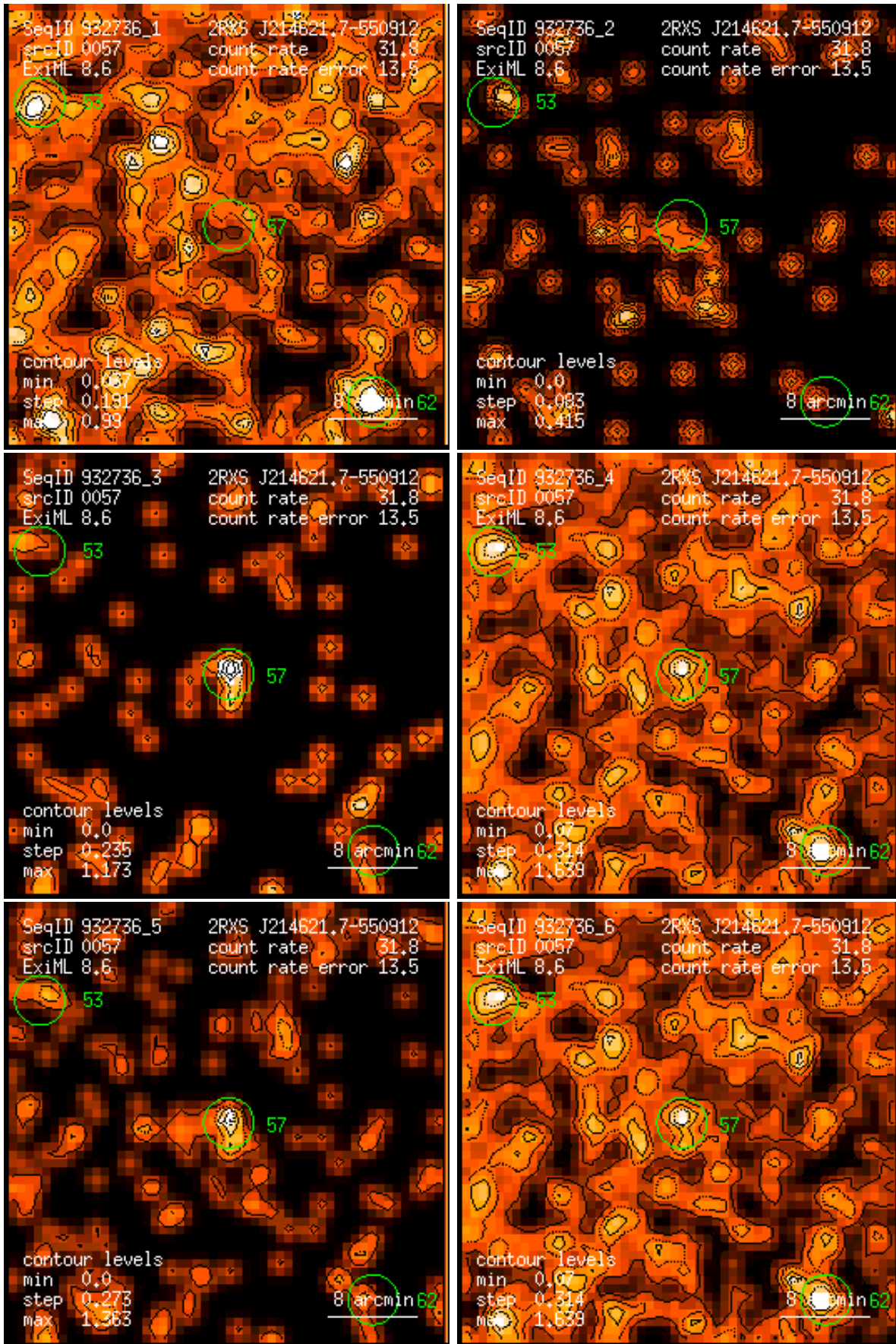
Figure 57: RASS 932736: detection 0057: band rate images, Gaussian filter: (1) PSPC channels 11 – 41, (2) 52 – 90, (3) 91 – 201, (4) 11 – 235, (5) 52 – 201, (6) 11 – 201. Broad band rates in counts/ks. Band rate contour levels in counts/ks/arcmin 2 .
