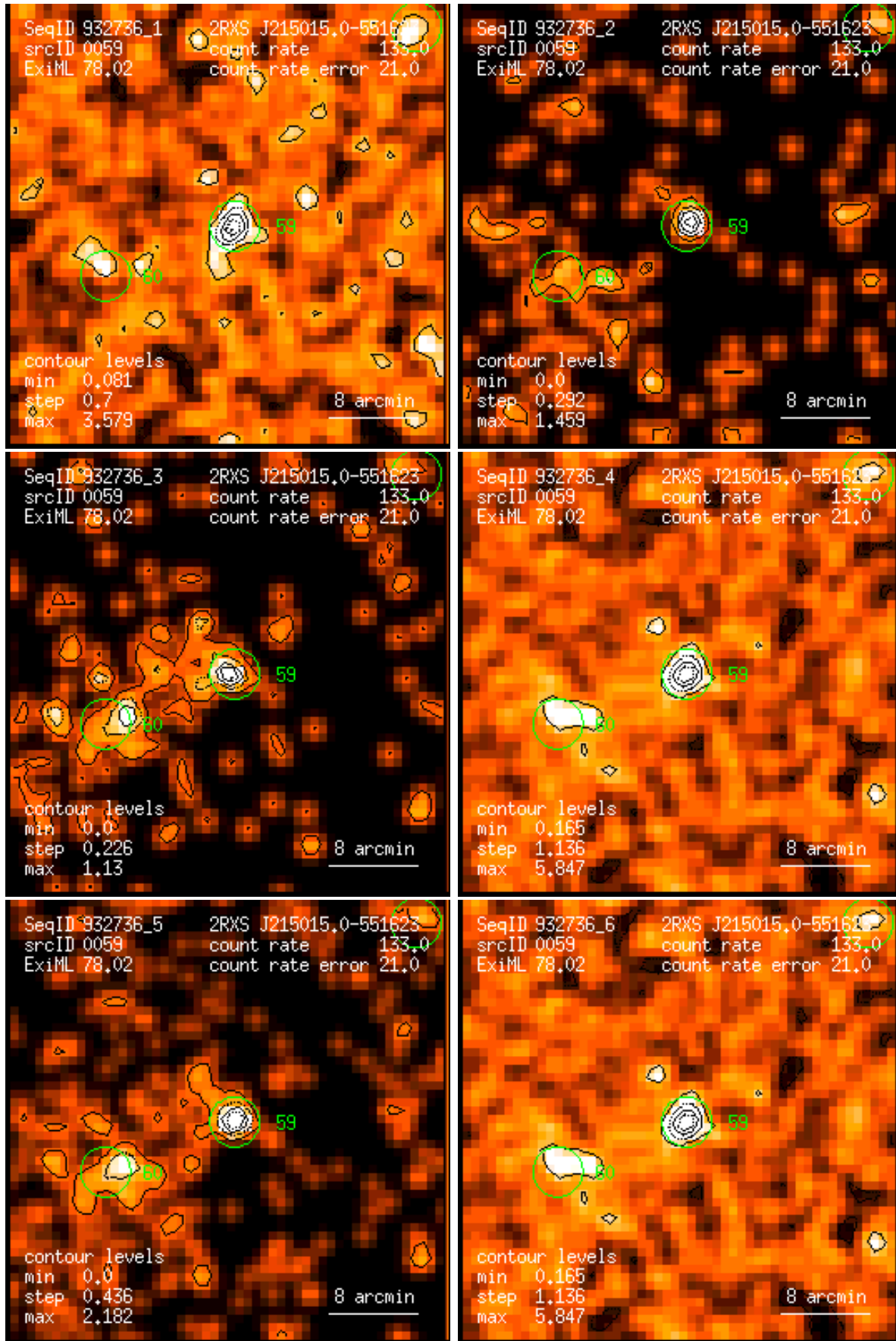
Figure 59: RASS 932736: detection 0059: band rate images, Gaussian filter: (1) PSPC channels 11 – 41, (2) 52 – 90, (3) 91 – 201, (4) 11 – 235, (5) 52 – 201, (6) 11 – 201. Broad band rates in counts/ks. Band rate contour levels in counts/ks/arcmin 2 .
