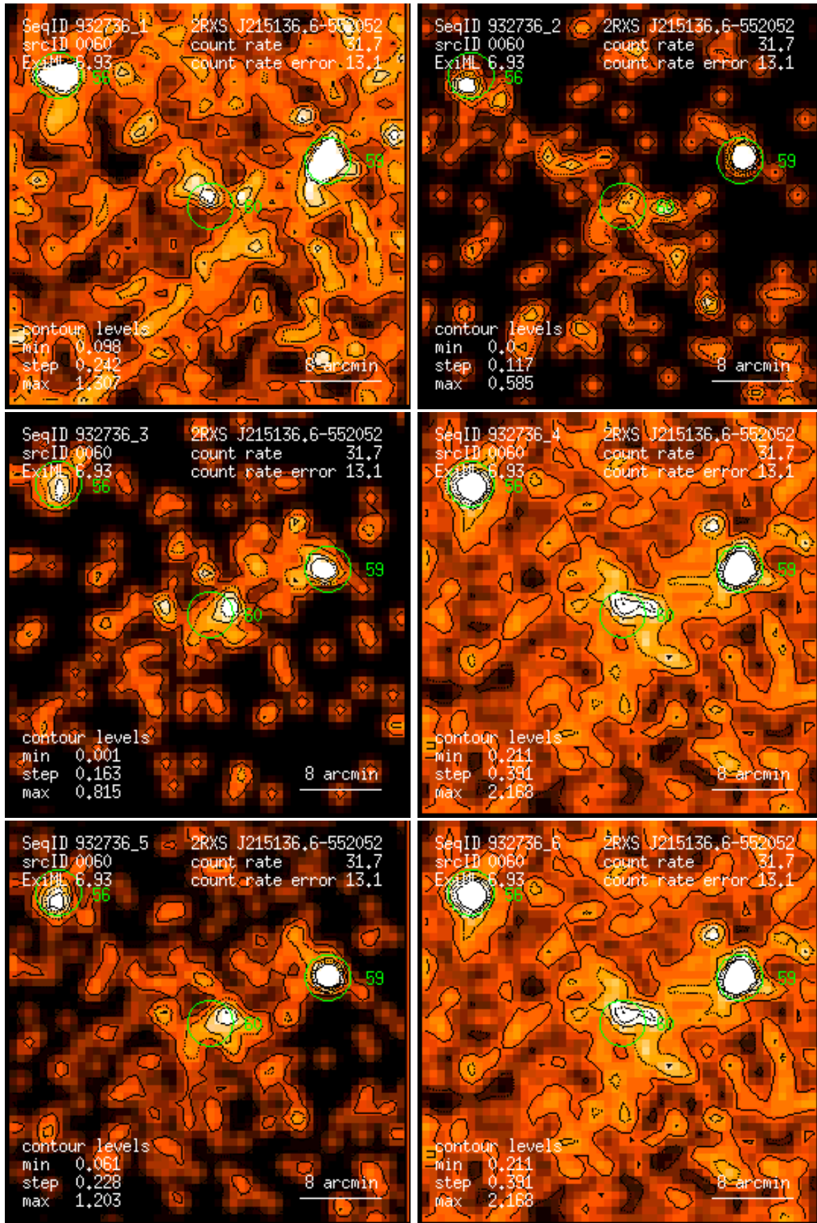
Figure 60: RASS 932736: detection 0060: band rate images, Gaussian filter: (1) PSPC channels 11 – 41, (2) 52 – 90, (3) 91 – 201, (4) 11 – 235, (5) 52 – 201, (6) 11 – 201. Broad band rates in counts/ks. Band rate contour levels in counts/ks/arcmin 2 .
