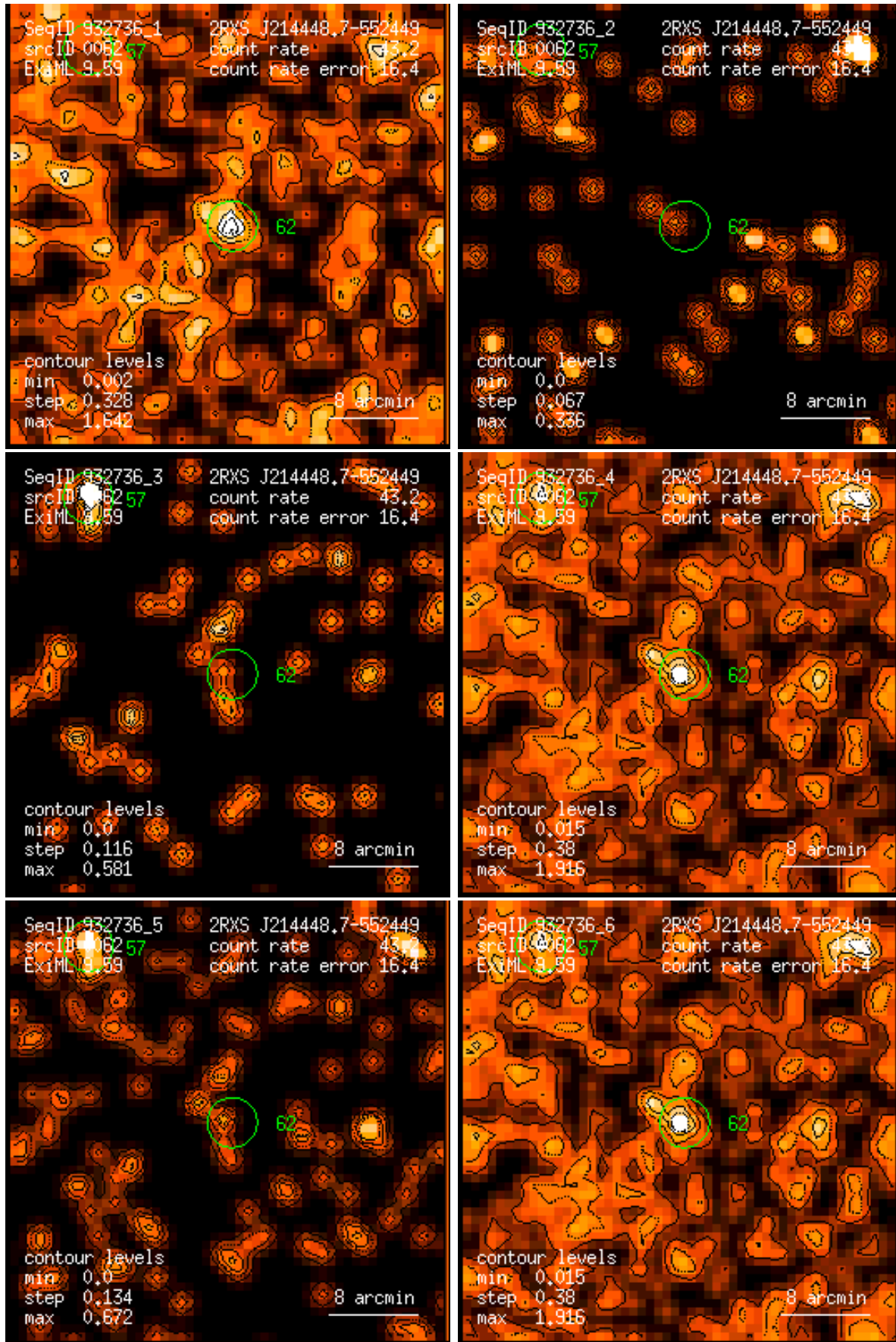
Figure 62: RASS 932736: detection 0062: band rate images, Gaussian filter: (1) PSPC channels 11 – 41, (2) 52 – 90, (3) 91 – 201, (4) 11 – 235, (5) 52 – 201, (6) 11 – 201. Broad band rates in counts/ks. Band rate contour levels in counts/ks/arcmin 2 .
