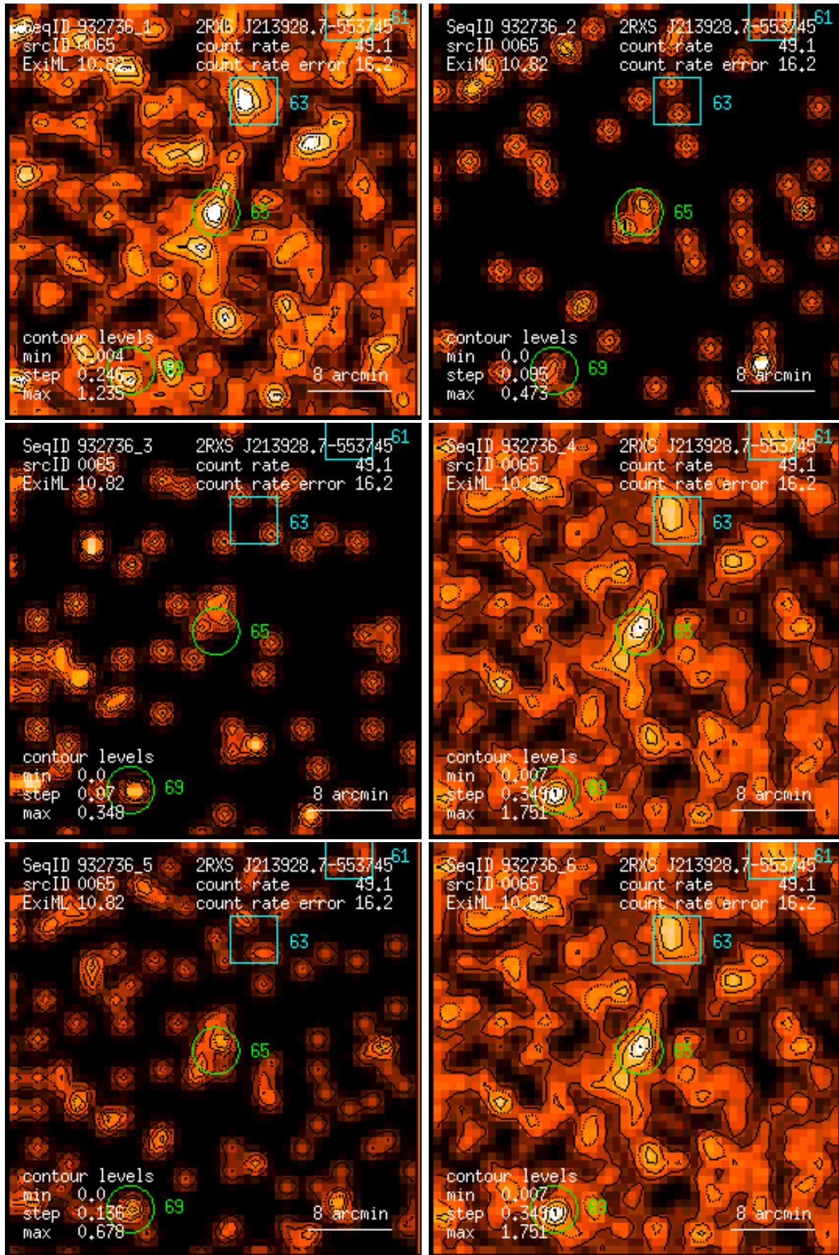
Figure 65: RASS 932736: detection 0065: band rate images, Gaussian filter: (1) PSPC channels 11 – 41, (2) 52 – 90, (3) 91 – 201, (4) 11 – 235, (5) 52 – 201, (6) 11 – 201. Broad band rates in counts/ks. Band rate contour levels in counts/ks/arcmin 2 .
