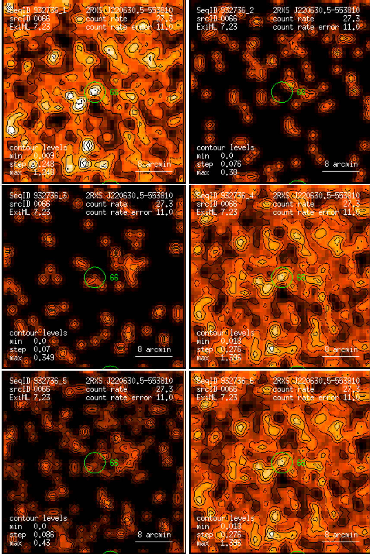
Figure 66: RASS 932736: detection 0066: band rate images, Gaussian filter: (1) PSPC channels 11 – 41, (2) 52 – 90, (3) 91 – 201, (4) 11 – 235, (5) 52 – 201, (6) 11 – 201. Broad band rates in counts/ks. Band rate contour levels in counts/ks/arcmin 2 .
