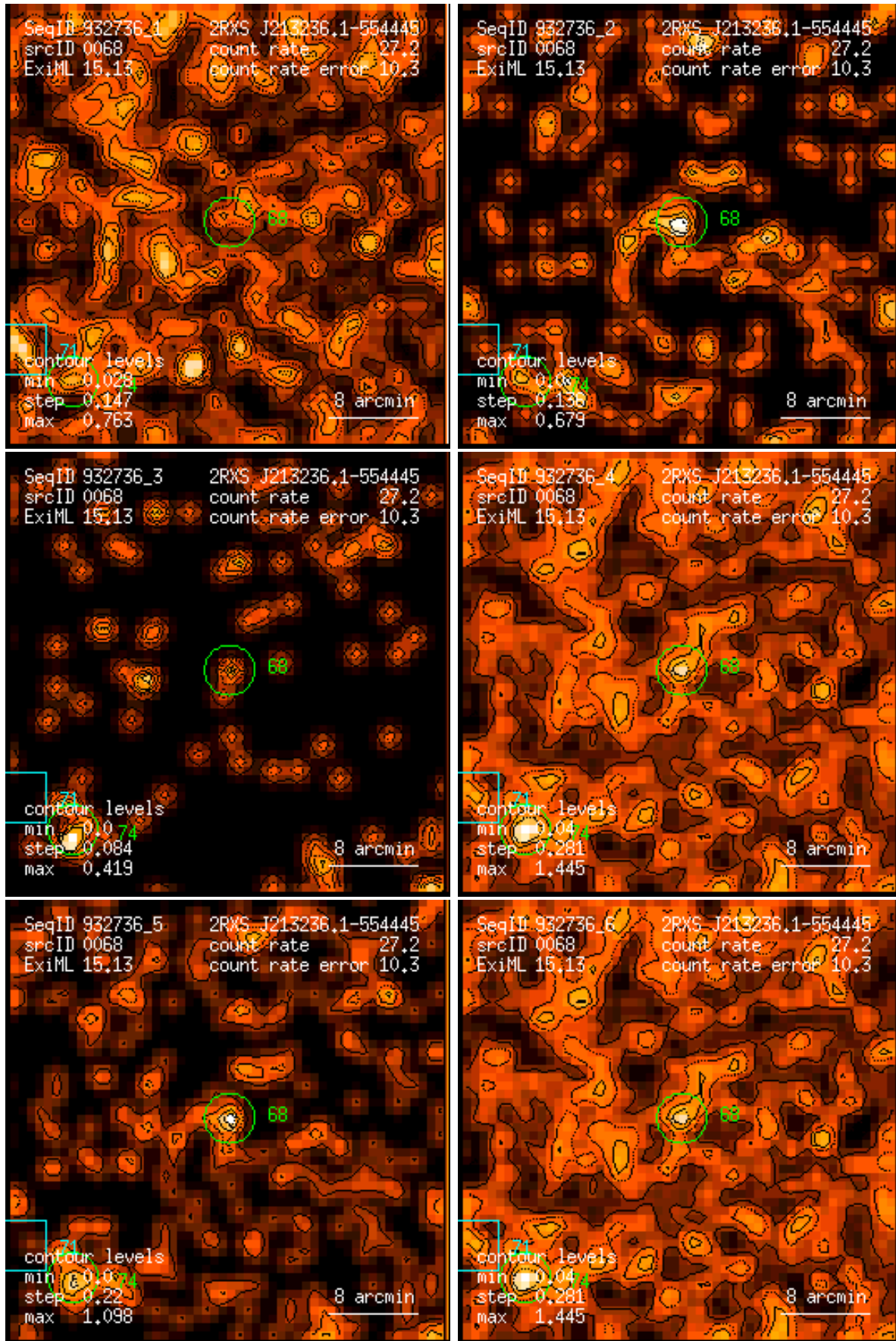
Figure 68: RASS 932736: detection 0068: band rate images, Gaussian filter: (1) PSPC channels 11 – 41, (2) 52 – 90, (3) 91 – 201, (4) 11 – 235, (5) 52 – 201, (6) 11 – 201. Broad band rates in counts/ks. Band rate contour levels in counts/ks/arcmin 2 .
