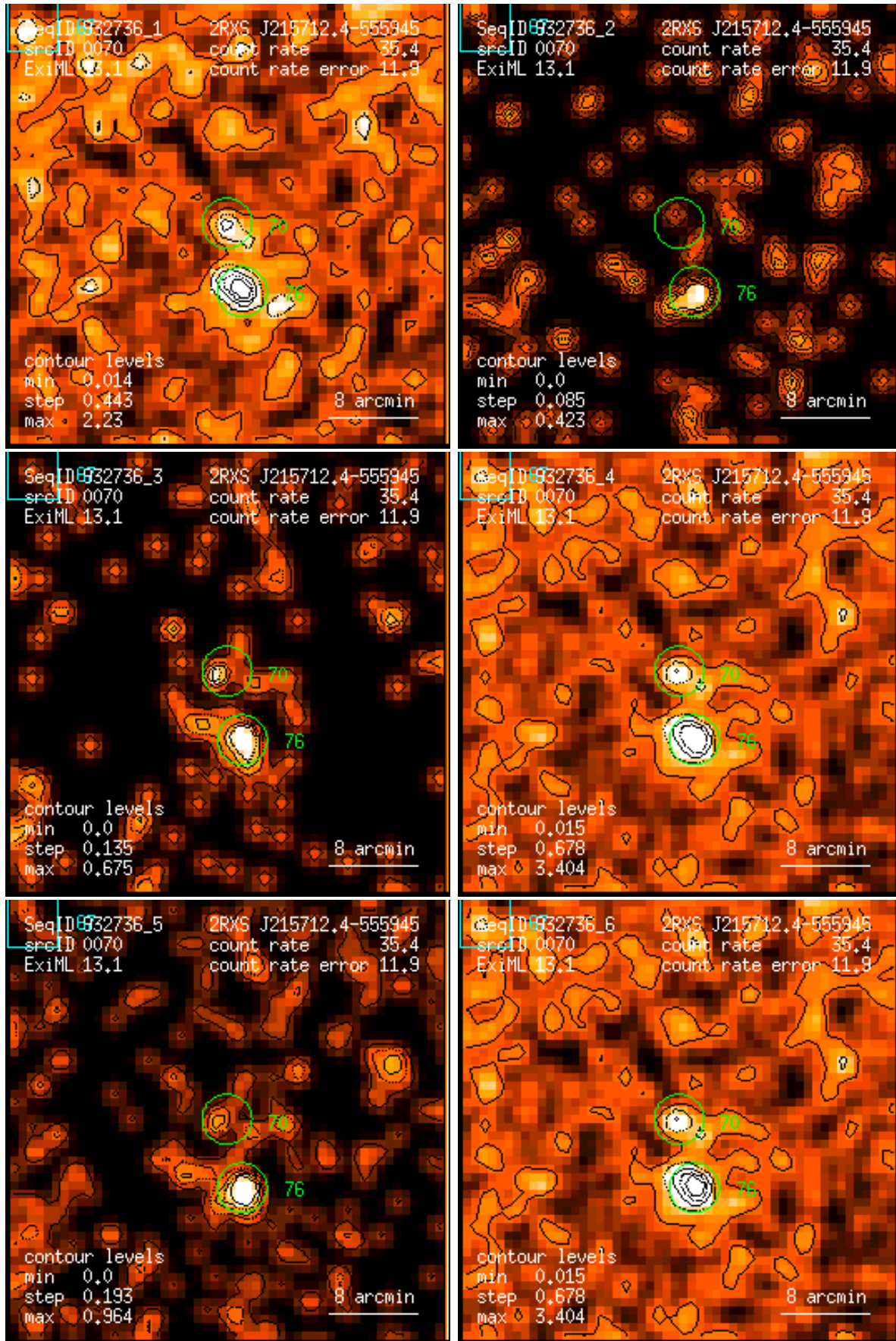
Figure 70: RASS 932736: detection 0070: band rate images, Gaussian filter: (1) PSPC channels 11 – 41, (2) 52 – 90, (3) 91 – 201, (4) 11 – 235, (5) 52 – 201, (6) 11 – 201. Broad band rates in counts/ks. Band rate contour levels in counts/ks/arcmin 2 .
