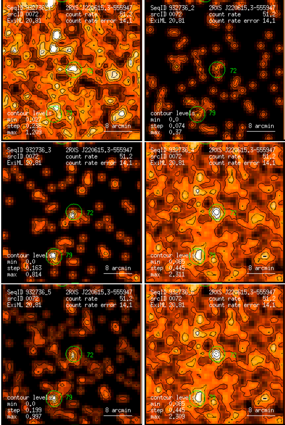
Figure 72: RASS 932736: detection 0072: band rate images, Gaussian filter: (1) PSPC channels 11 – 41, (2) 52 – 90, (3) 91 – 201, (4) 11 – 235, (5) 52 – 201, (6) 11 – 201. Broad band rates in counts/ks. Band rate contour levels in counts/ks/arcmin 2 .
