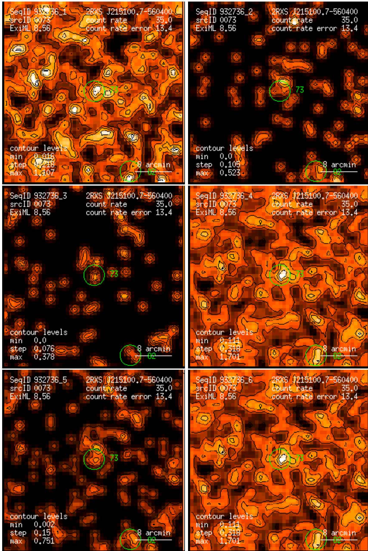
Figure 73: RASS 932736: detection 0073: band rate images, Gaussian filter: (1) PSPC channels 11 – 41, (2) 52 – 90, (3) 91 – 201, (4) 11 – 235, (5) 52 – 201, (6) 11 – 201. Broad band rates in counts/ks. Band rate contour levels in counts/ks/arcmin 2 .
