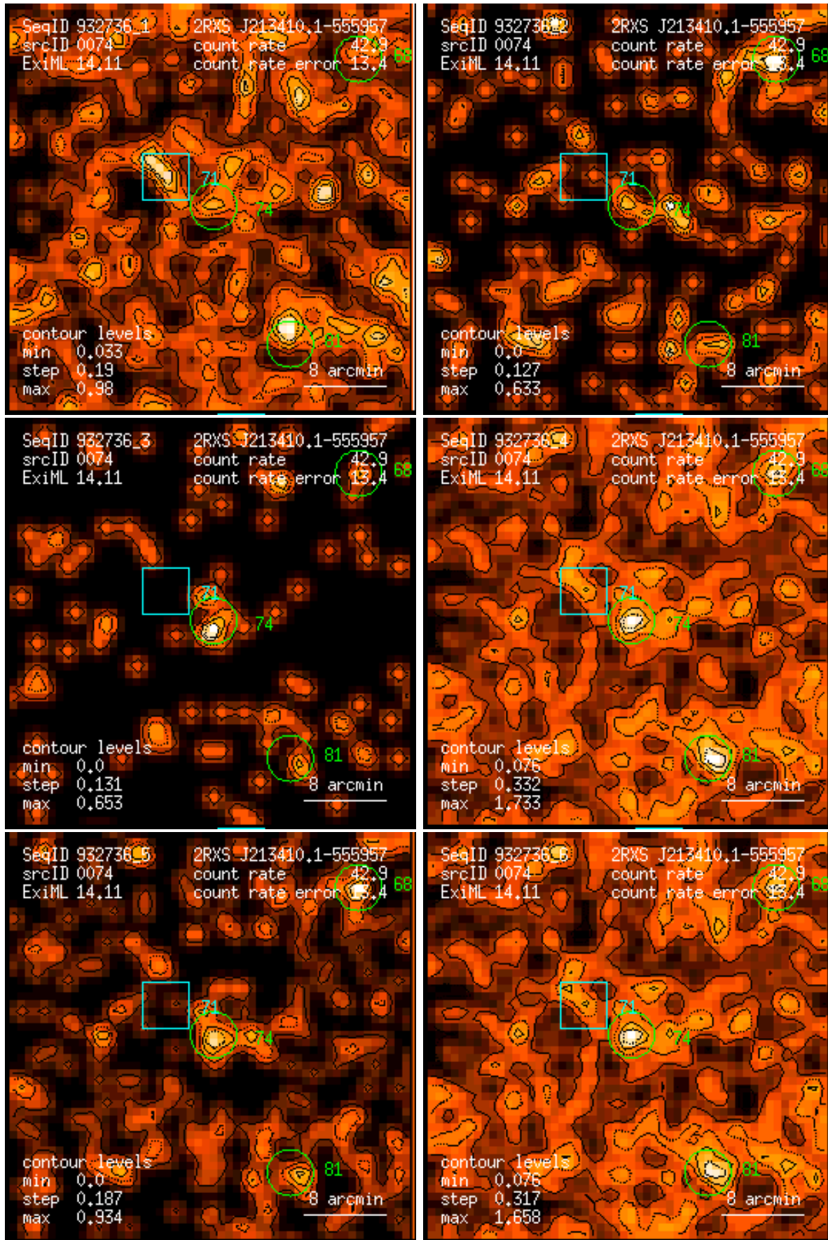
Figure 74: RASS 932736: detection 0074: band rate images, Gaussian filter: (1) PSPC channels 11 – 41, (2) 52 – 90, (3) 91 – 201, (4) 11 – 235, (5) 52 – 201, (6) 11 – 201. Broad band rates in counts/ks. Band rate contour levels in counts/ks/arcmin 2 .
