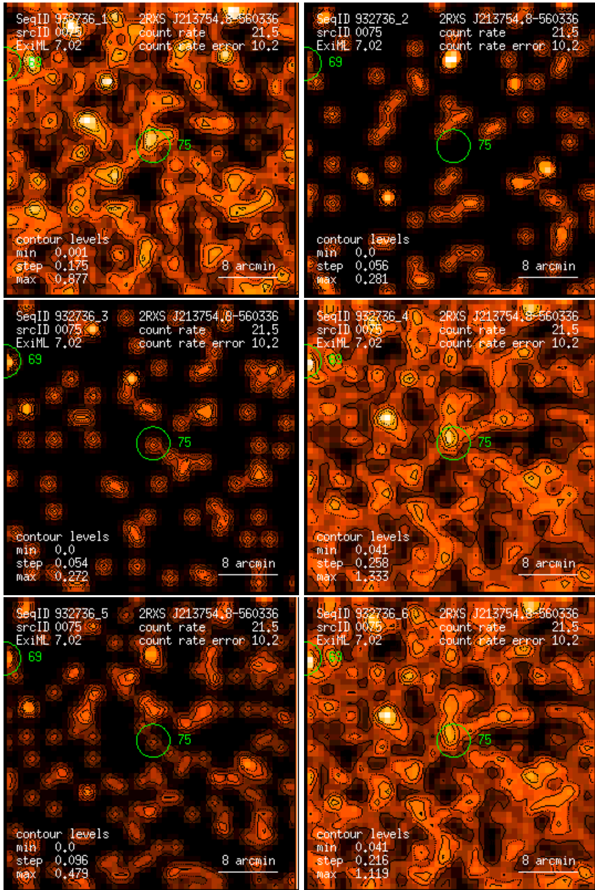
Figure 75: RASS 932736: detection 0075: band rate images, Gaussian filter: (1) PSPC channels 11 – 41, (2) 52 – 90, (3) 91 – 201, (4) 11 – 235, (5) 52 – 201, (6) 11 – 201. Broad band rates in counts/ks. Band rate contour levels in counts/ks/arcmin 2 .
