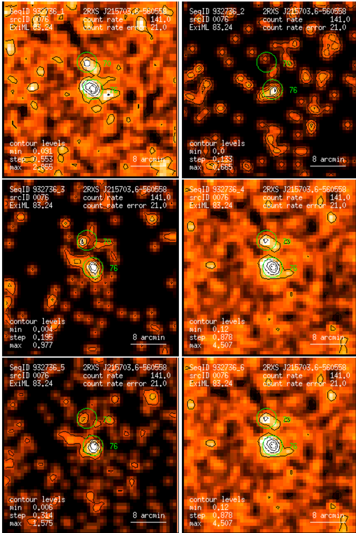
Figure 76: RASS 932736: detection 0076: band rate images, Gaussian filter: (1) PSPC channels 11 – 41, (2) 52 – 90, (3) 91 – 201, (4) 11 – 235, (5) 52 – 201, (6) 11 – 201. Broad band rates in counts/ks. Band rate contour levels in counts/ks/arcmin 2 .
