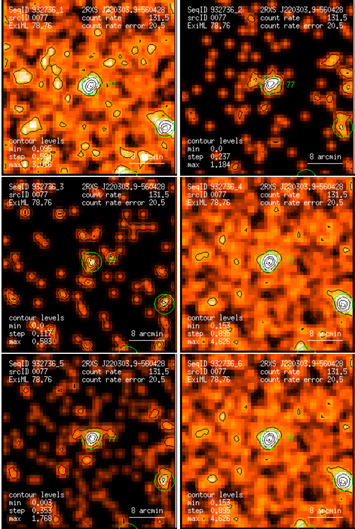
Figure 77: RASS 932736: detection 0077: band rate images, Gaussian filter: (1) PSPC channels 11 – 41, (2) 52 – 90, (3) 91 – 201, (4) 11 – 235, (5) 52 – 201, (6) 11 – 201. Broad band rates in counts/ks. Band rate contour levels in counts/ks/arcmin 2 .
