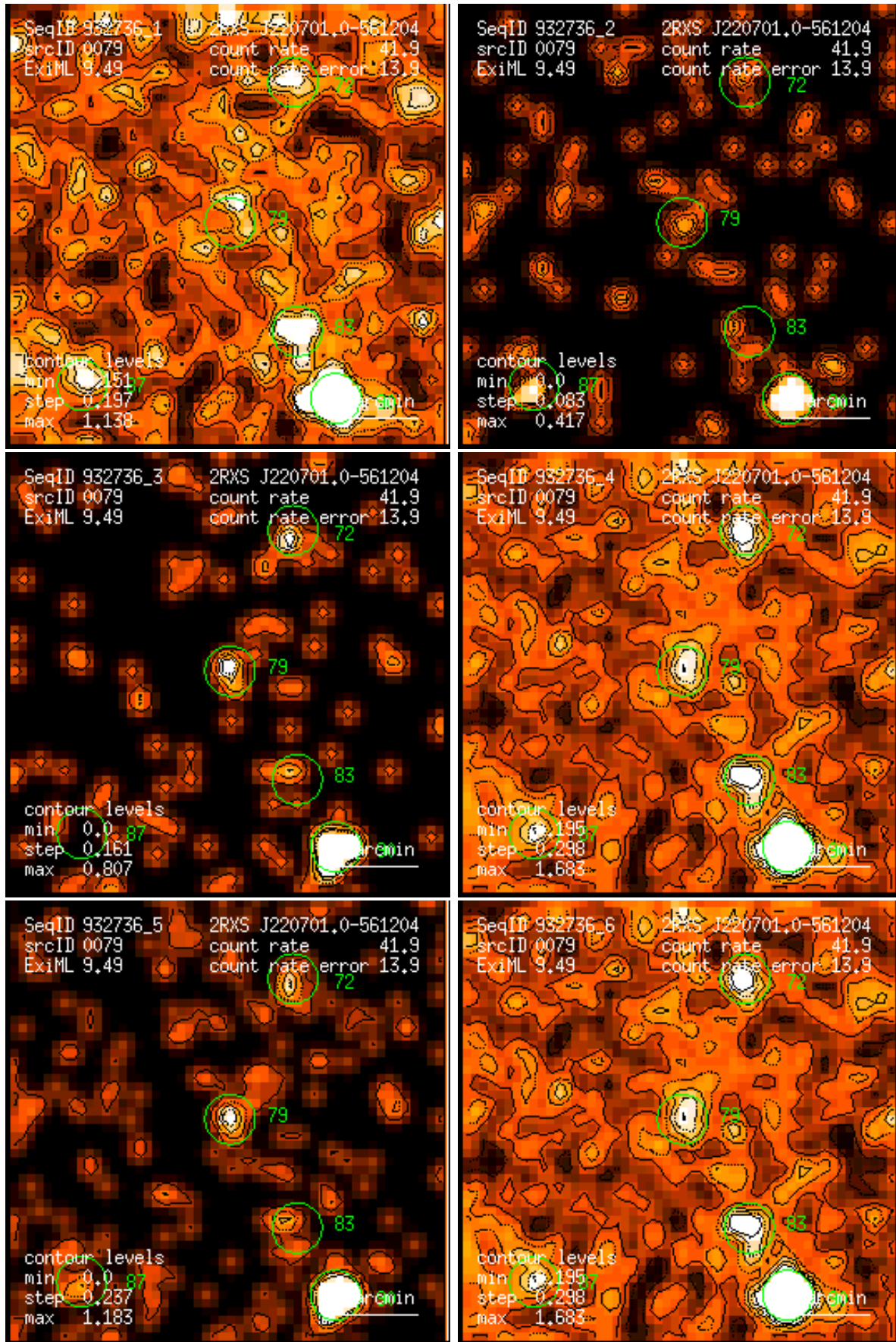
Figure 79: RASS 932736: detection 0079: band rate images, Gaussian filter: (1) PSPC channels 11 – 41, (2) 52 – 90, (3) 91 – 201, (4) 11 – 235, (5) 52 – 201, (6) 11 – 201. Broad band rates in counts/ks. Band rate contour levels in counts/ks/arcmin 2 .
