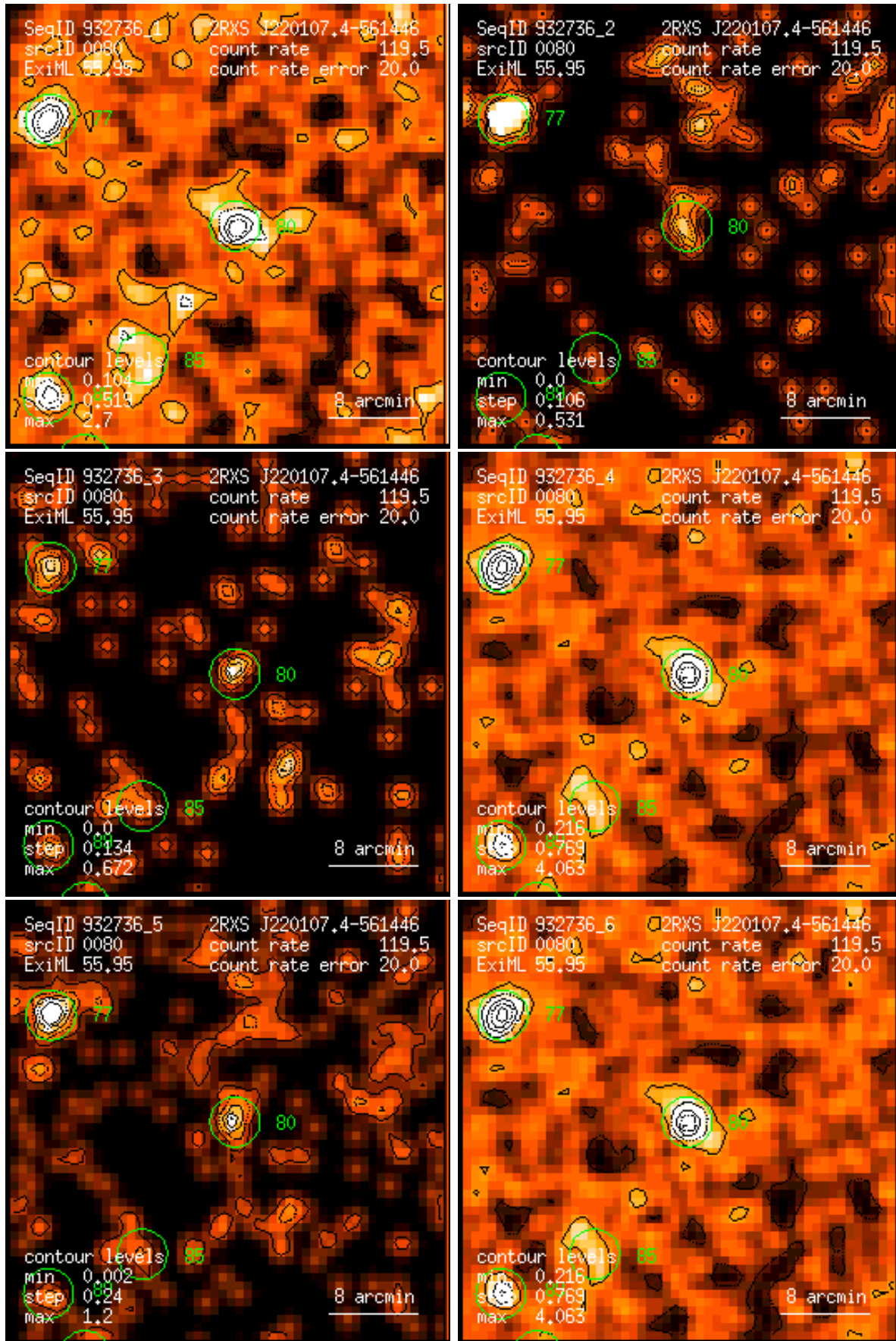
Figure 80: RASS 932736: detection 0080: band rate images, Gaussian filter: (1) PSPC channels 11 – 41, (2) 52 – 90, (3) 91 – 201, (4) 11 – 235, (5) 52 – 201, (6) 11 – 201. Broad band rates in counts/ks. Band rate contour levels in counts/ks/arcmin 2 .
