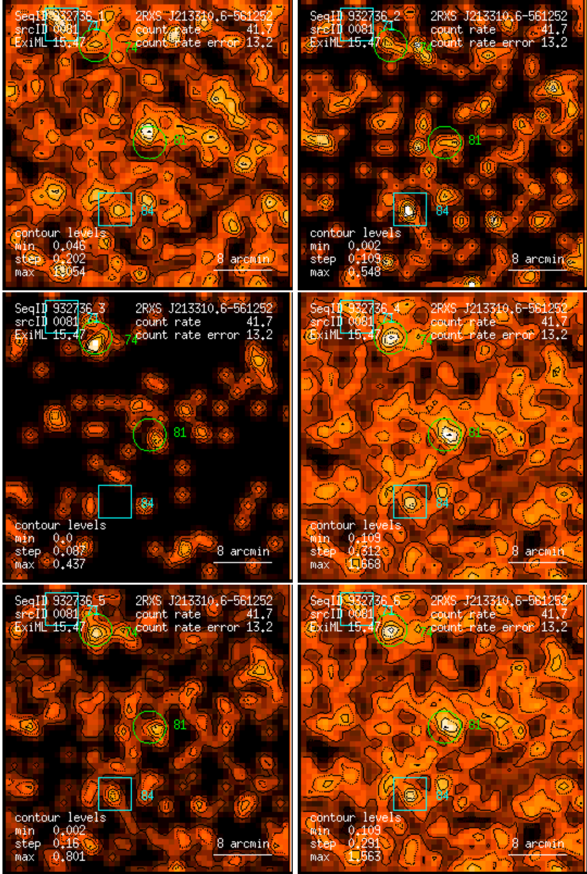
Figure 81: RASS 932736: detection 0081: band rate images, Gaussian filter: (1) PSPC channels 11 – 41, (2) 52 – 90, (3) 91 – 201, (4) 11 – 235, (5) 52 – 201, (6) 11 – 201. Broad band rates in counts/ks. Band rate contour levels in counts/ks/arcmin 2 .
