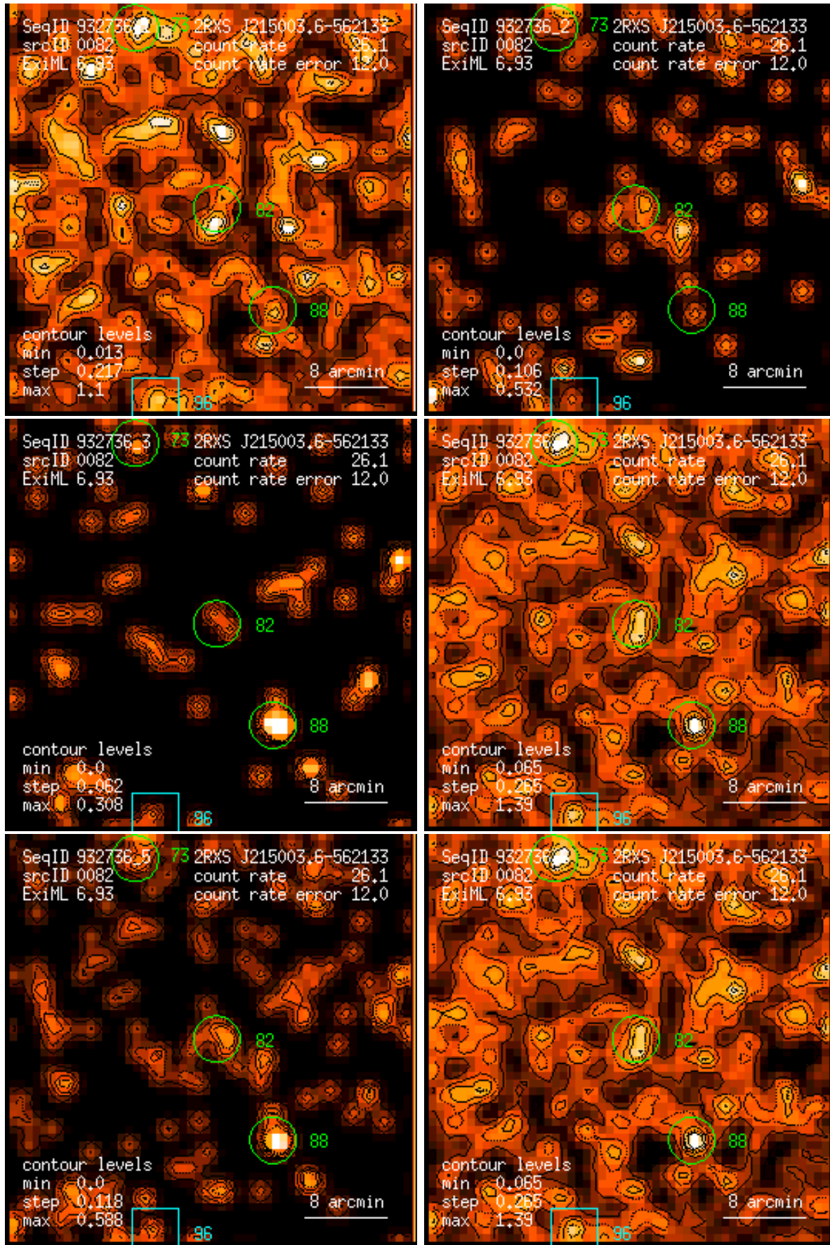
Figure 82: RASS 932736: detection 0082: band rate images, Gaussian filter: (1) PSPC channels 11 – 41, (2) 52 – 90, (3) 91 – 201, (4) 11 – 235, (5) 52 – 201, (6) 11 – 201. Broad band rates in counts/ks. Band rate contour levels in counts/ks/arcmin 2 .
