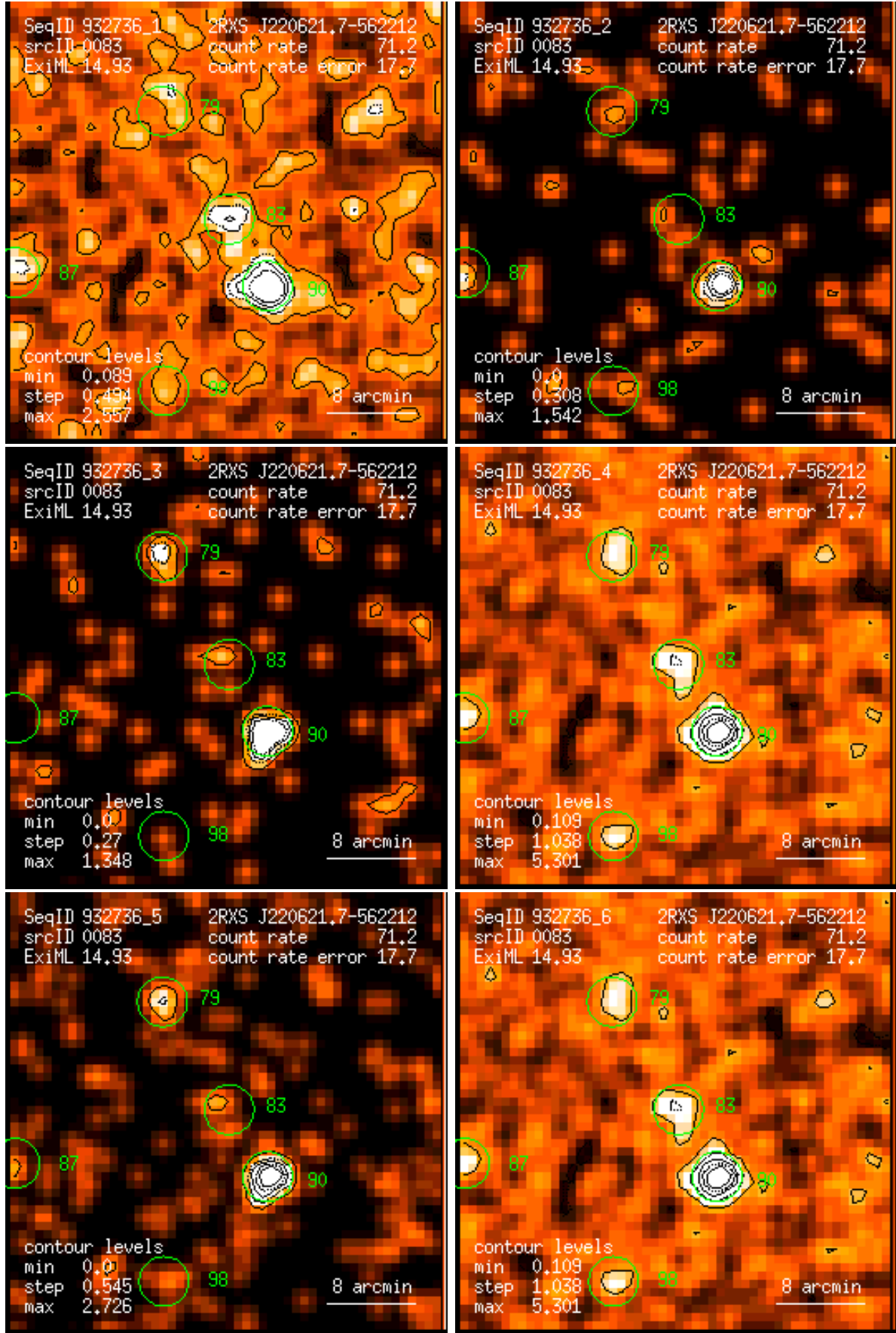
Figure 83: RASS 932736: detection 0083: band rate images, Gaussian filter: (1) PSPC channels 11 – 41, (2) 52 – 90, (3) 91 – 201, (4) 11 – 235, (5) 52 – 201, (6) 11 – 201. Broad band rates in counts/ks. Band rate contour levels in counts/ks/arcmin 2 .
