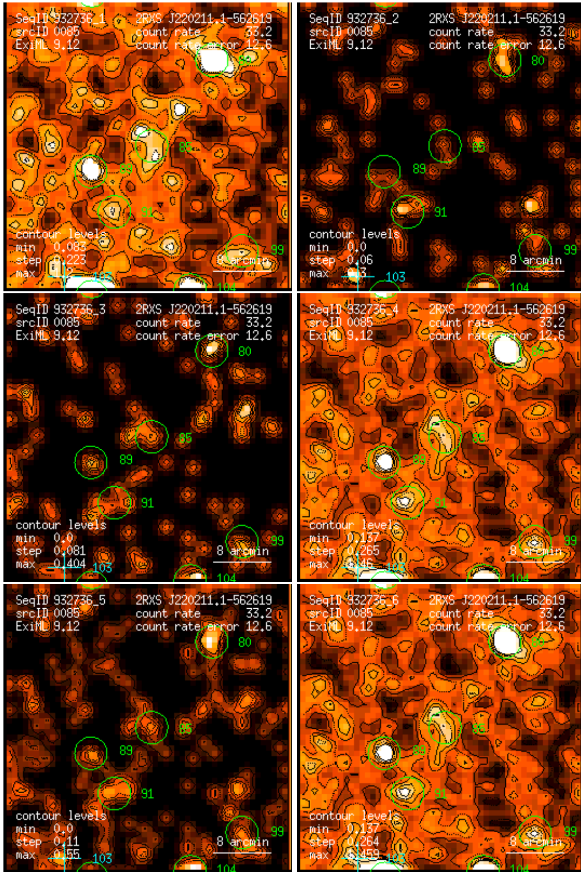
Figure 85: RASS 932736: detection 0085: band rate images, Gaussian filter: (1) PSPC channels 11 – 41, (2) 52 – 90, (3) 91 – 201, (4) 11 – 235, (5) 52 – 201, (6) 11 – 201. Broad band rates in counts/ks. Band rate contour levels in counts/ks/arcmin 2 .
