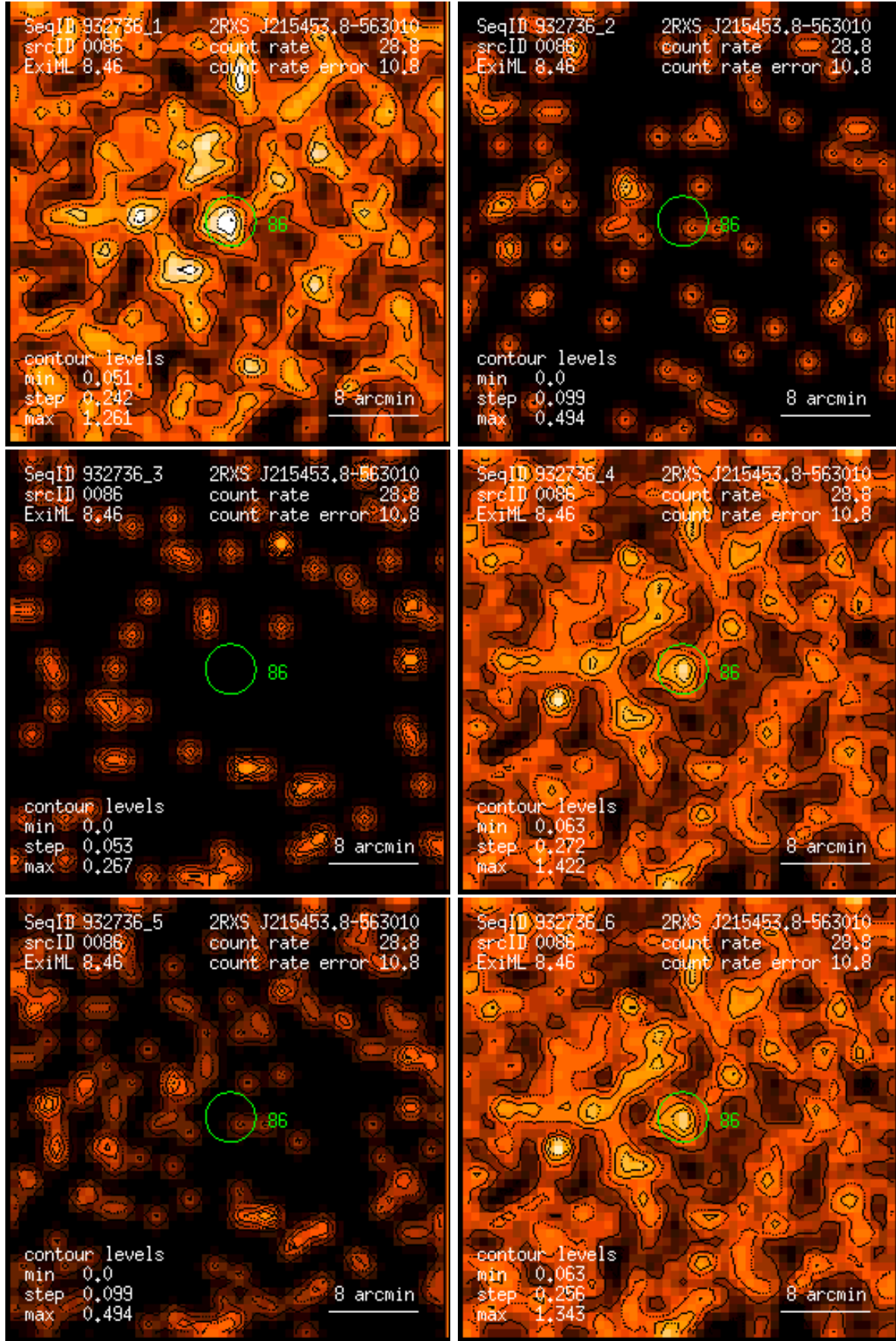
Figure 86: RASS 932736: detection 0086: band rate images, Gaussian filter: (1) PSPC channels 11 – 41, (2) 52 – 90, (3) 91 – 201, (4) 11 – 235, (5) 52 – 201, (6) 11 – 201. Broad band rates in counts/ks. Band rate contour levels in counts/ks/arcmin 2 .
