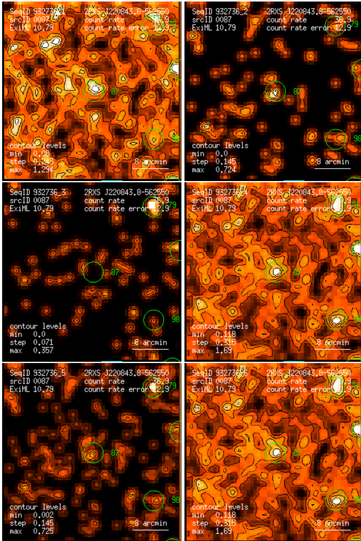
Figure 87: RASS 932736: detection 0087: band rate images, Gaussian filter: (1) PSPC channels 11 – 41, (2) 52 – 90, (3) 91 – 201, (4) 11 – 235, (5) 52 – 201, (6) 11 – 201. Broad band rates in counts/ks. Band rate contour levels in counts/ks/arcmin 2 .
