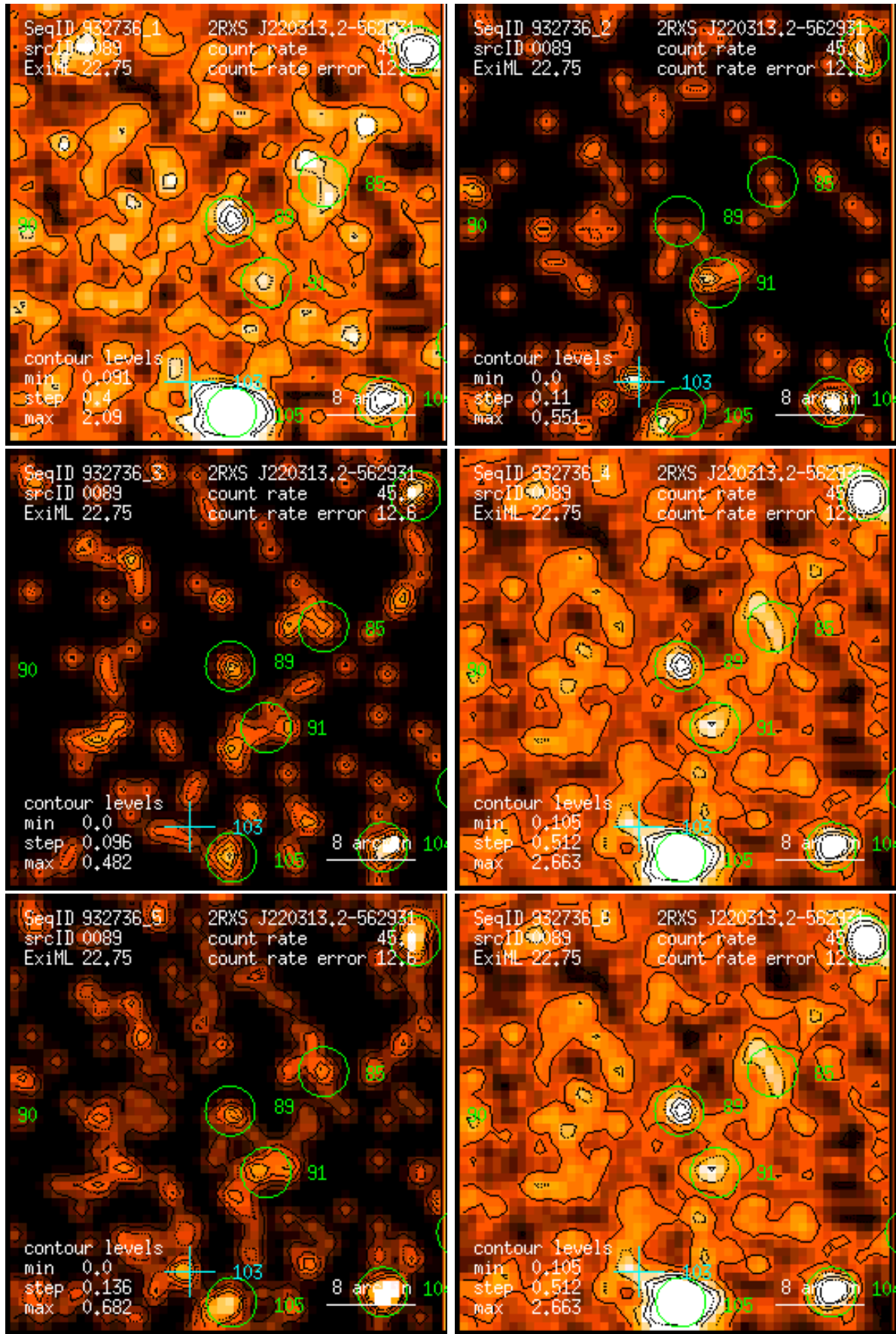
Figure 89: RASS 932736: detection 0089: band rate images, Gaussian filter: (1) PSPC channels 11 – 41, (2) 52 – 90, (3) 91 – 201, (4) 11 – 235, (5) 52 – 201, (6) 11 – 201. Broad band rates in counts/ks. Band rate contour levels in counts/ks/arcmin 2 .
