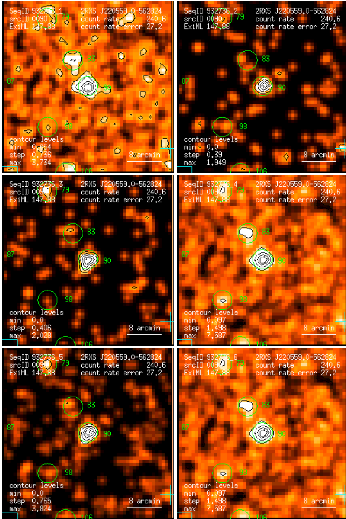
Figure 90: RASS 932736: detection 0090: band rate images, Gaussian filter: (1) PSPC channels 11 – 41, (2) 52 – 90, (3) 91 – 201, (4) 11 – 235, (5) 52 – 201, (6) 11 – 201. Broad band rates in counts/ks. Band rate contour levels in counts/ks/arcmin 2 .
