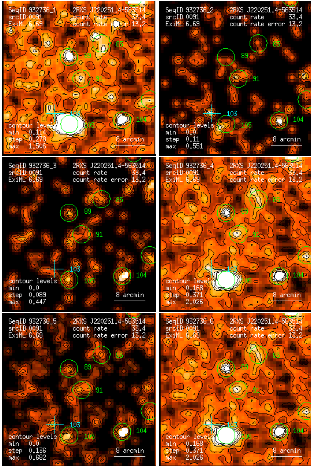
Figure 91: RASS 932736: detection 0091: band rate images, Gaussian filter: (1) PSPC channels 11 – 41, (2) 52 – 90, (3) 91 – 201, (4) 11 – 235, (5) 52 – 201, (6) 11 – 201. Broad band rates in counts/ks. Band rate contour levels in counts/ks/arcmin 2 .
