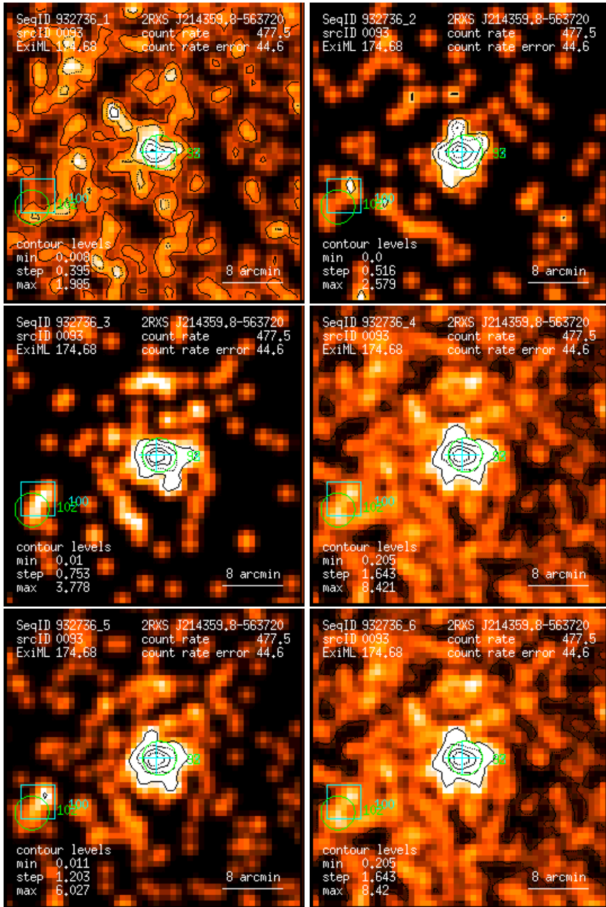
Figure 93: RASS 932736: detection 0093: band rate images, Gaussian filter: (1) PSPC channels 11 – 41, (2) 52 – 90, (3) 91 – 201, (4) 11 – 235, (5) 52 – 201, (6) 11 – 201. Broad band rates in counts/ks. Band rate contour levels in counts/ks/arcmin 2 .
