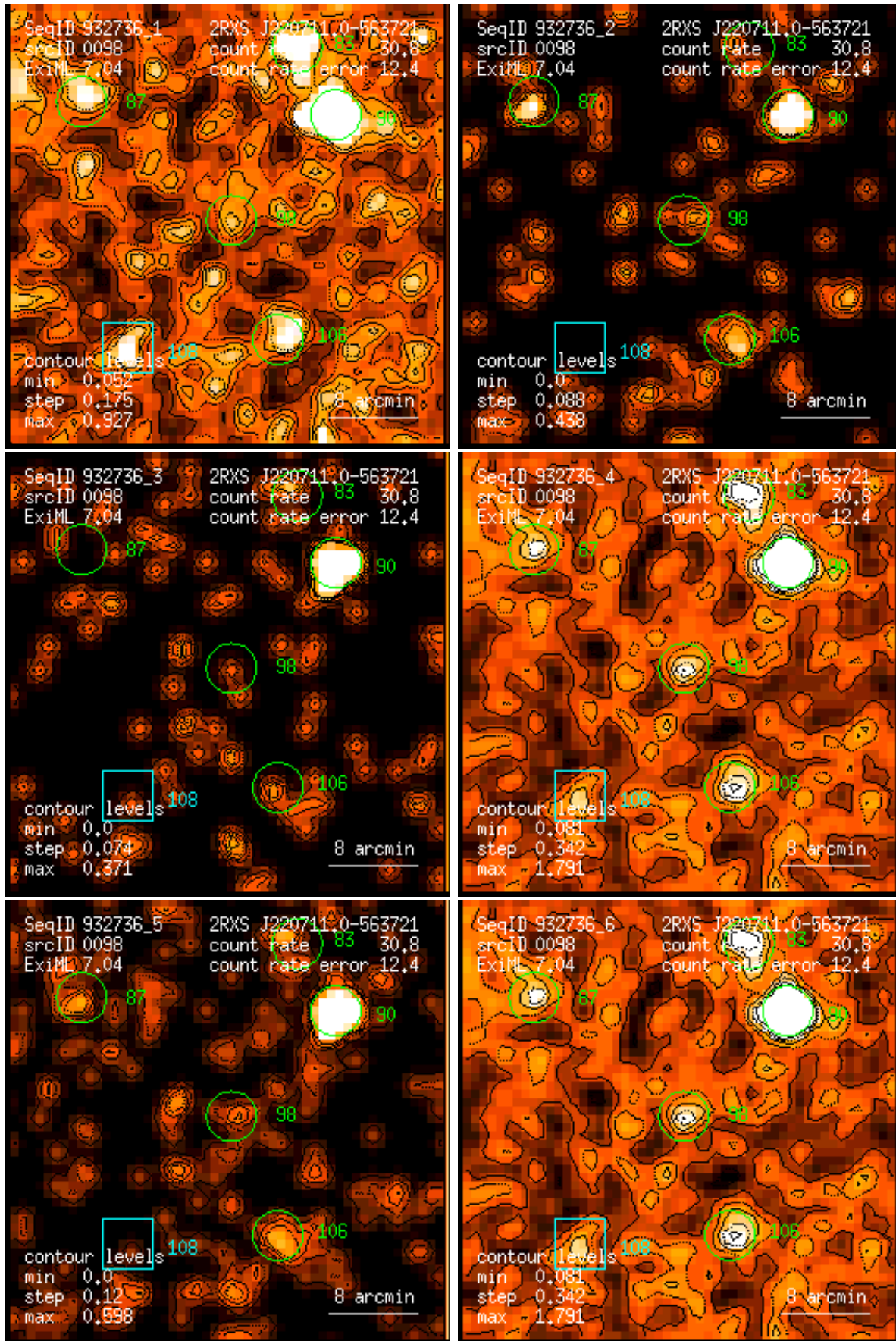
Figure 98: RASS 932736: detection 0098: band rate images, Gaussian filter: (1) PSPC channels 11 – 41, (2) 52 – 90, (3) 91 – 201, (4) 11 – 235, (5) 52 – 201, (6) 11 – 201. Broad band rates in counts/ks. Band rate contour levels in counts/ks/arcmin 2 .
