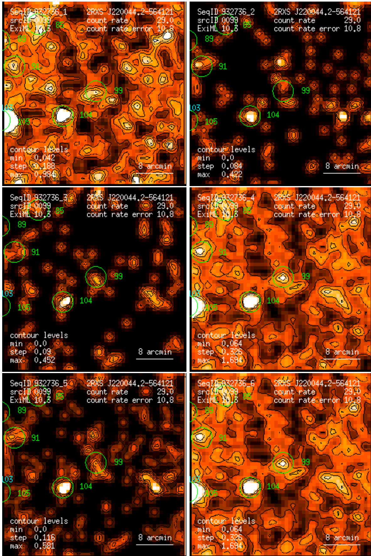
Figure 99: RASS 932736: detection 0099: band rate images, Gaussian filter: (1) PSPC channels 11 – 41, (2) 52 – 90, (3) 91 – 201, (4) 11 – 235, (5) 52 – 201, (6) 11 – 201. Broad band rates in counts/ks. Band rate contour levels in counts/ks/arcmin 2 .
