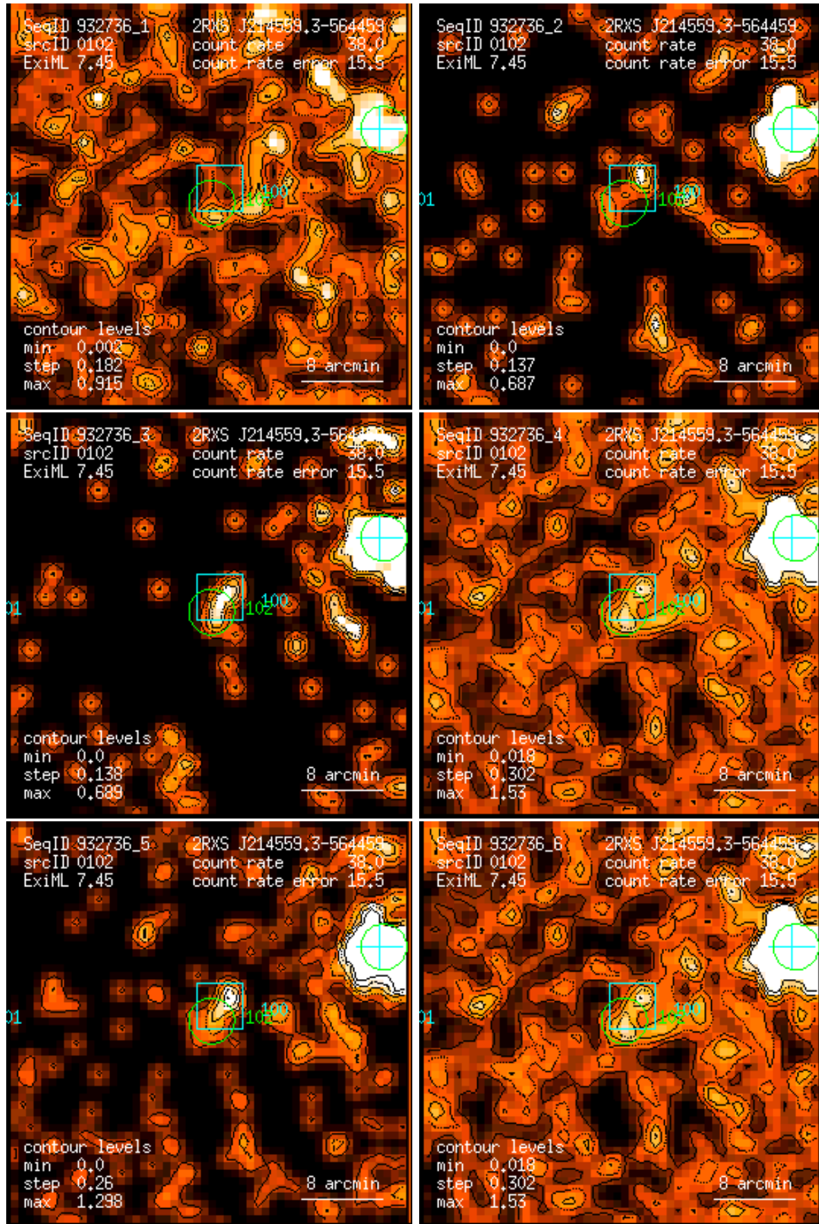
Figure 102: RASS 932736: detection 0102: band rate images, Gaussian filter: (1) PSPC channels 11 – 41, (2) 52 – 90, (3) 91 – 201, (4) 11 – 235, (5) 52 – 201, (6) 11 – 201. Broad band rates in counts/ks. Band rate contour levels in counts/ks/arcmin 2 .
