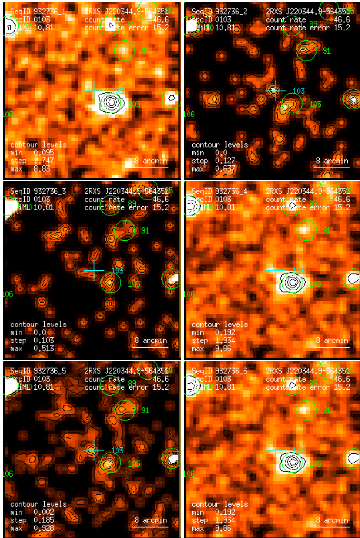
Figure 103: RASS 932736: detection 0103: band rate images, Gaussian filter: (1) PSPC channels 11 – 41, (2) 52 – 90, (3) 91 – 201, (4) 11 – 235, (5) 52 – 201, (6) 11 – 201. Broad band rates in counts/ks. Band rate contour levels in counts/ks/arcmin 2 .
