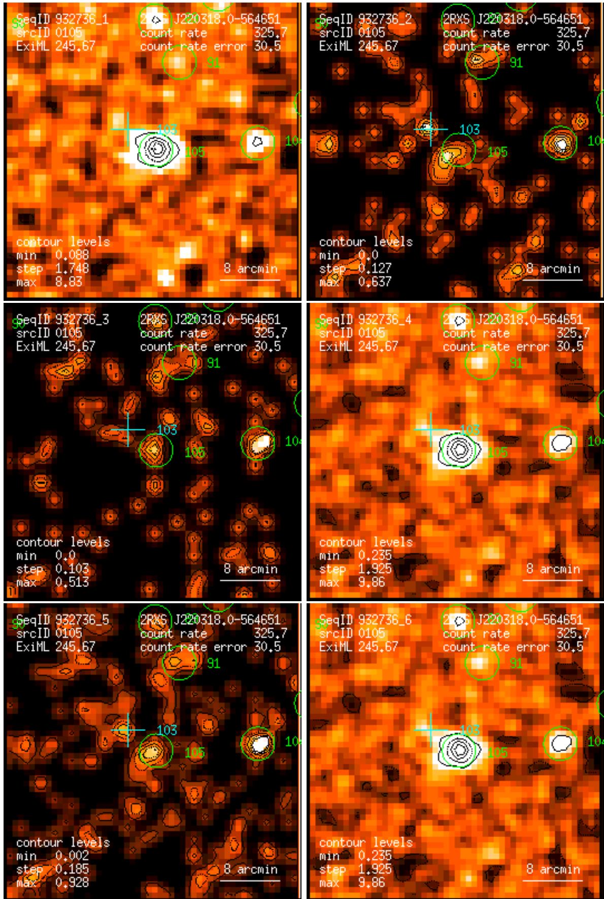
Figure 105: RASS 932736: detection 0105: band rate images, Gaussian filter: (1) PSPC channels 11 – 41, (2) 52 – 90, (3) 91 – 201, (4) 11 – 235, (5) 52 – 201, (6) 11 – 201. Broad band rates in counts/ks. Band rate contour levels in counts/ks/arcmin 2 .
