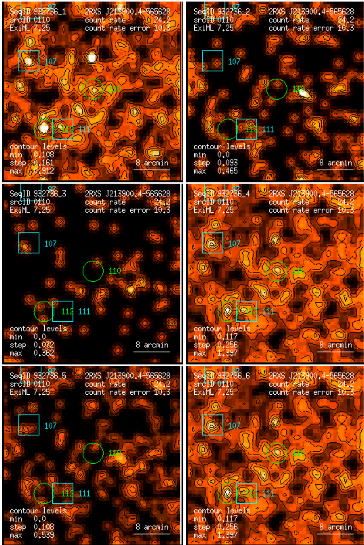
Figure 110: RASS 932736: detection 0110: band rate images, Gaussian filter: (1) PSPC channels 11 – 41, (2) 52 – 90, (3) 91 – 201, (4) 11 – 235, (5) 52 – 201, (6) 11 – 201. Broad band rates in counts/ks. Band rate contour levels in counts/ks/arcmin 2 .
