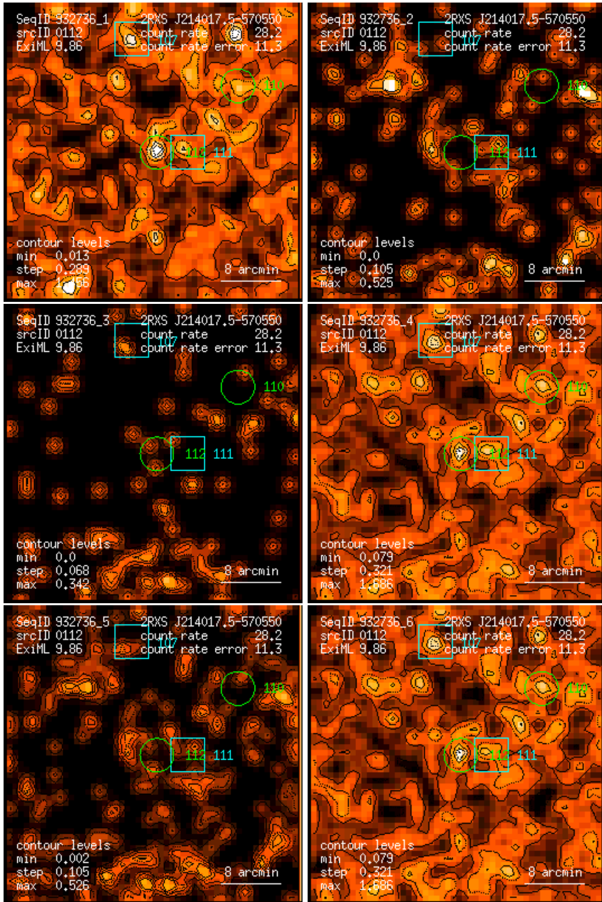
Figure 112: RASS 932736: detection 0112: band rate images, Gaussian filter: (1) PSPC channels 11 – 41, (2) 52 – 90, (3) 91 – 201, (4) 11 – 235, (5) 52 – 201, (6) 11 – 201. Broad band rates in counts/ks. Band rate contour levels in counts/ks/arcmin 2 .
